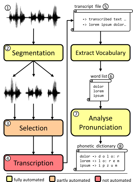
Fig. 6. Workflow for extending our speech corpus.
