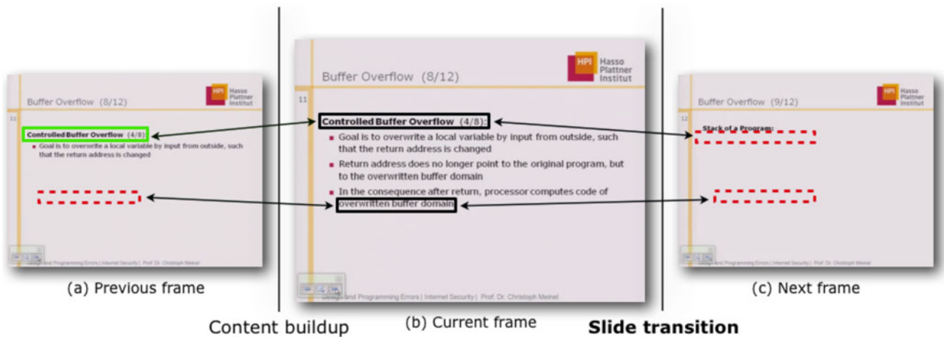
Fig. 2. We detect the first and the last object line in R_c vertically and perform the CC differencing metric on those line sequences from adjacent frames. In frame (a) and (b), a same text line (top) can be found; whereas in frame (b) and (c), the CC-based differences of both text lines exceed the threshold T_{s2} . A slide transition is thus found between frame (b) and (c).
