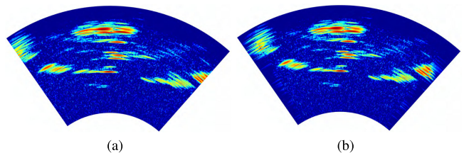
Fig. 9. Comparison of the incomplete echo data and extrapolated echo data. (a) Incomplete echo data. (b) Extrapolated complete echo data.
