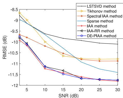
Fig. 7. Influence of echo SNR on scene edge target.
