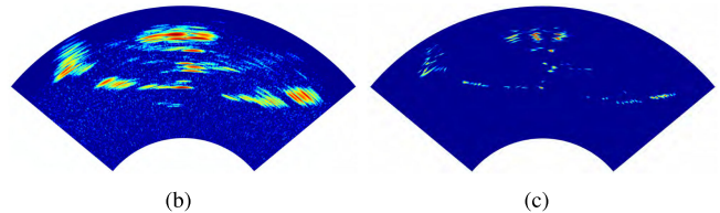
Fig. 8. Experimental scenario and echo data. (a) Experimental scenario. (b) Echo data. (c) Super-resolution result.
