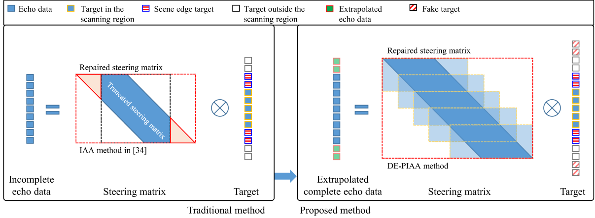
Fig. 2. Process diagram.
