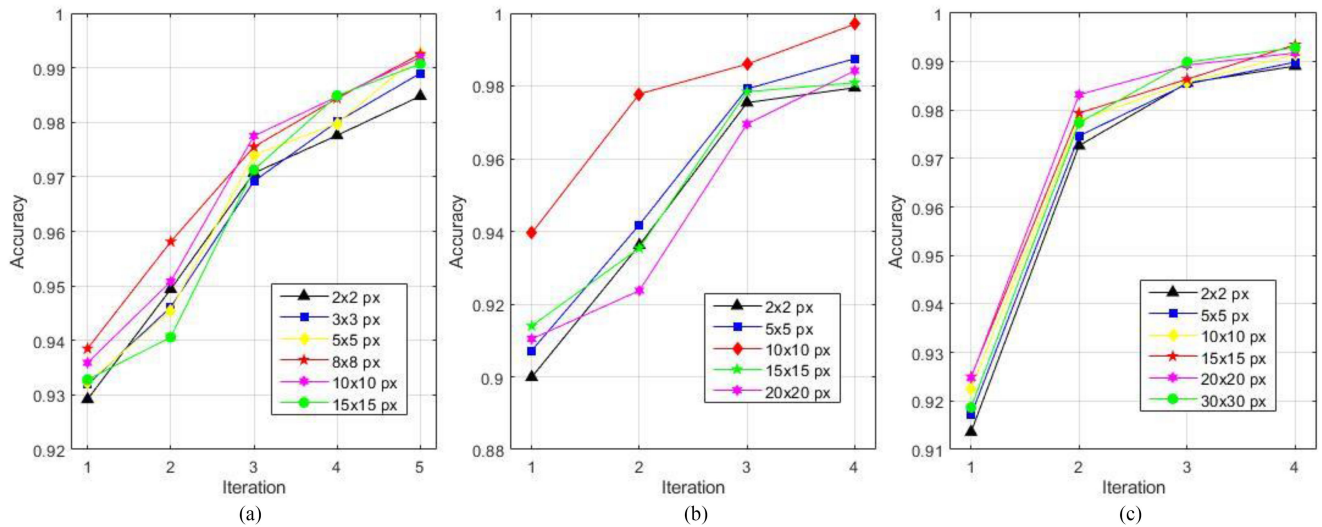
Fig. 10. Comparison of change detection accuracies conducting different iterations in the proposed approach with various scene scales. (a) Landsat 5 dataset. (b) Sentinel-2 dataset. (c) UAV dataset.
