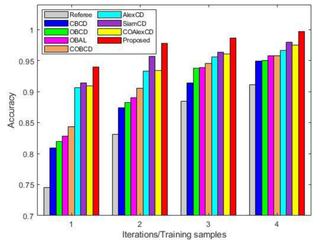
Fig. 7. Comparison of different change detection results of Sentinel-2 dataset with increasing number of training samples.
