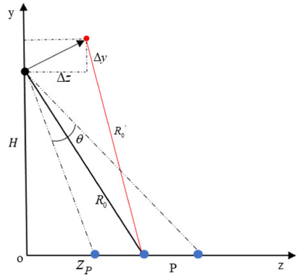
Fig. 3. LOS displacement in the cross-track plane.
