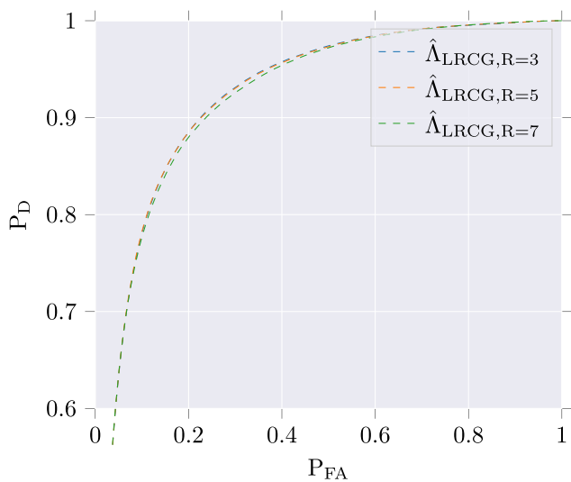
Fig. 12. Comparison for the scene 1 of the LRCG for different rank values. The window size is fixed at 7 \times 7 and \sigma^2 is assumed unknown.
