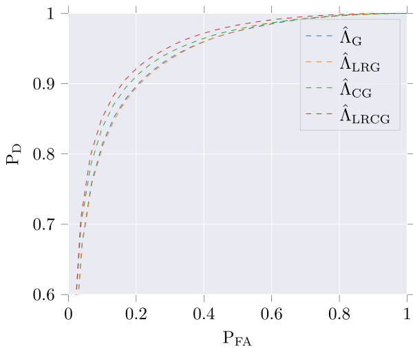
Fig. 10. Comparison between four methods for the scene 2: Gaussian, LR Gaussian, CG, and LRCG. Rank is fixed as 3, the window size is 7 \times 7 and \sigma^2 is assumed unknown for LR models.
