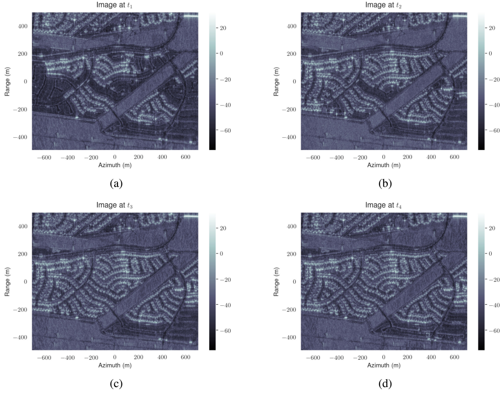
Fig. 2. UAVSAR dataset used in this study for the scene 1. Four dates are available between April 23, 2009 and May 15, 2011. (a) t = 1 . (b) t = 2 . (c) t = 3 . (d) t = 4 .
