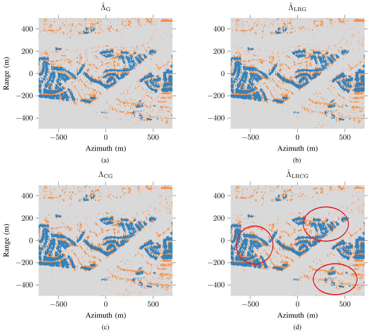
Fig. 8. Thresholded outputs of the four methods for the scene 1 for a fixed probability of false alarm (10%): true detection in blue and false alarms in orange. Rank is fixed as 3, the window size is 7 \times 7 and \sigma^2 is assumed unknown for both LR models. (a) Gaussian. (b) LR Gaussian. (c) CG. (d) LR CG.
