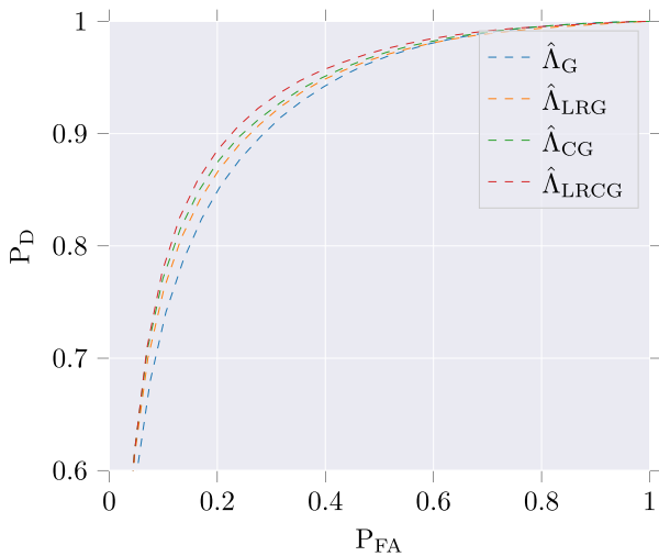
Fig. 7. Comparison between four methods for the scene 1: Gaussian, LR Gaussian, CG, and LRCG. Rank is fixed as 3, the window size is 7 \times 7 and \sigma^2 is assumed unknown for both LR models.
