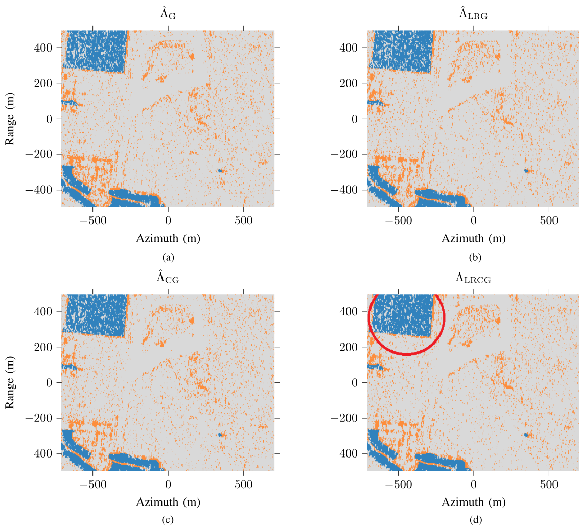
Fig. 11. Thresholded outputs of the four methods for the scene 2 for a fixed probability of false alarm (10%): true detection in blue and false alarms in orange. Rank is fixed as 3, the window size is 7 \times 7 and \sigma^2 is assumed unknown for both LR models. (a) Gaussian. (b) LR Gaussian. (c) CG. (d) LRCG.
