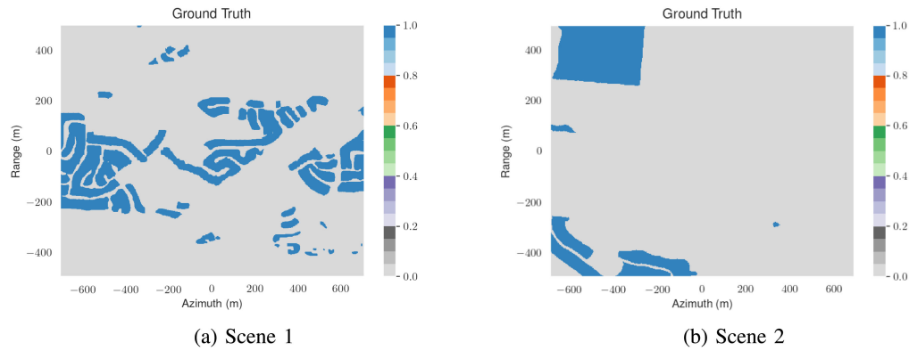
Fig. 4. Ground truth for scenes 1 and 2. (a) Scene 1. (b) Scene 2.
