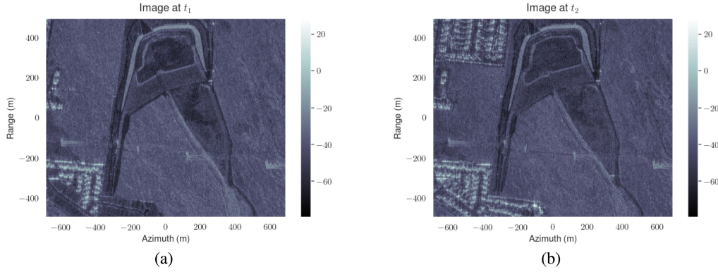
Fig. 3. UAVSAR dataset used in this study for the scene 2. Two dates are available between April 23, 2009 and May 15, 2011. (a) t = 1 . (b) t = 2 .
