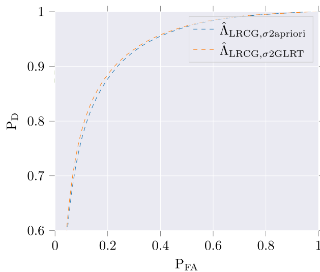
Fig. 13. Comparison for the scene 1 of the LRCG with assumed known \sigma^2 and assumed unknown \sigma^2 (integrated in GLRT). R = 3 , Window size is equal to 7 \times 7 .
