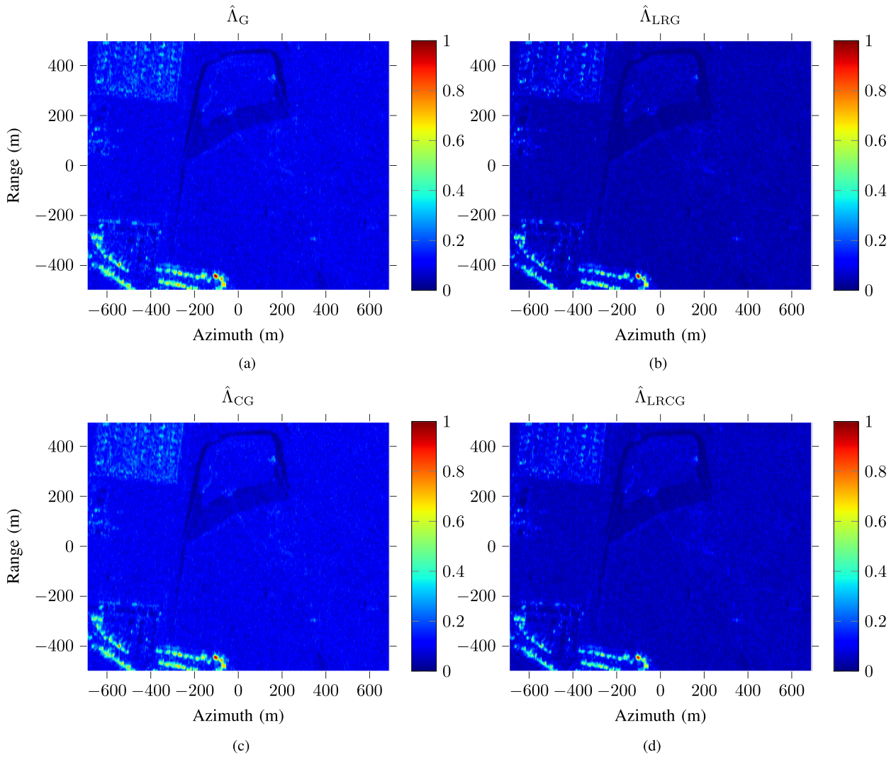
Fig. 9. Outputs of the four methods for the scene 2. (a) Gaussian. (b) LR Gaussian. (c) CG. (d) LRCG. Rank is fixed as 3, the window size is 7 \times 7 and \sigma^2 is assumed unknown for LR models.
