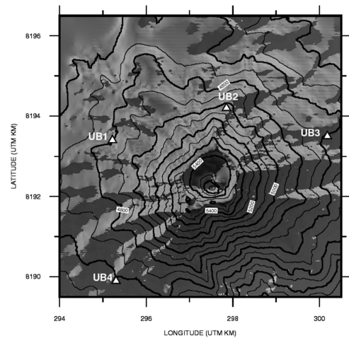
Fig. 2. Map of the Ubina volcano with the UB1, UB2, UB3, and UB4 permanent stations.
