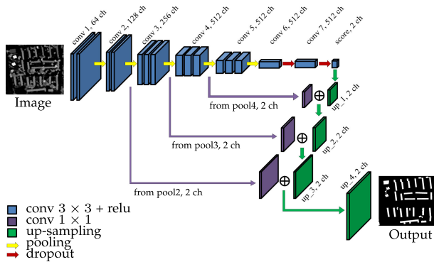
Fig. 1. Schematic representation of our FCN4s architecture.
