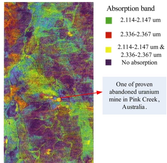
Fig. 14. Pine Creek Uranium mine investigation by MAIS data. The yellow color represents the uranium deposit extracted by using the Spectral Absorption Index with data in wavelength 2.114–2.147 \mu\text{m} and 2.336–2.367 \mu\text{m} .
