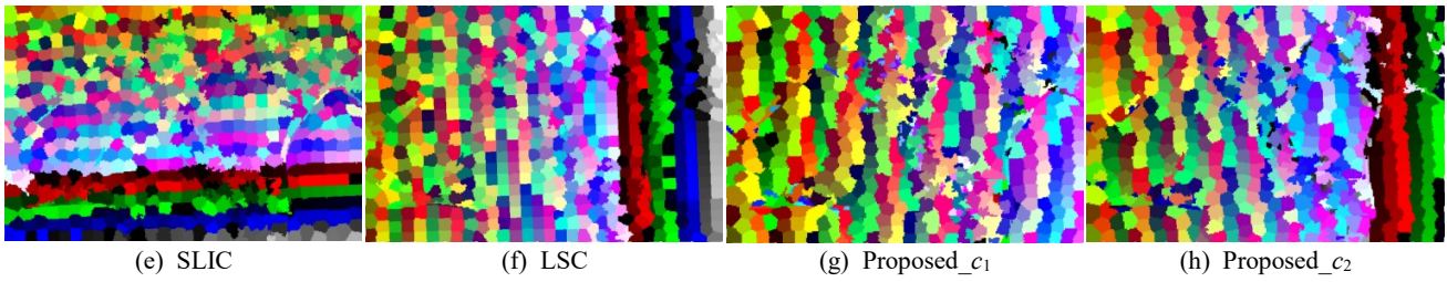
Fig.7. Superpixel segmentation results of Landsat8, (a) NCut, (b) ERS, (c) Turbopixels, (d) SCoW, (e) SLIC, (f) LSC, (g) Proposed algorithm based on c_1 diffusion coefficient, (h) Proposed algorithm based on c_2 diffusion coefficient.
