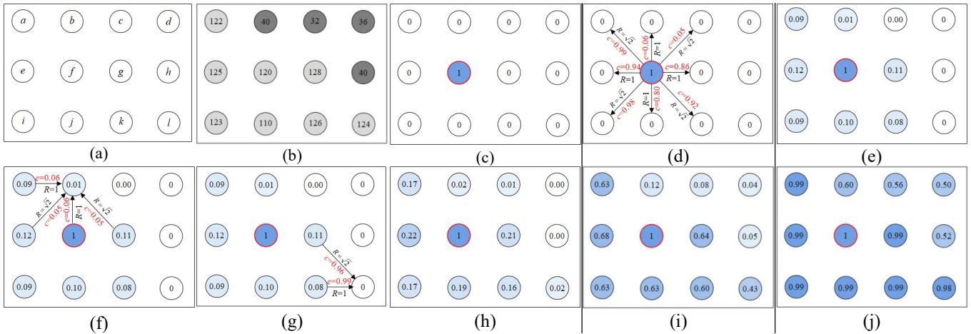
Fig.3. The concentration diffusion process with diffusion coefficient c_1 , (a) Index of pixel site, (b) Gray value of pixels, (c) Diffusion flux at the initial time (i.e. t=0 ) by assuming f as the seed point; (d) Diffusion state at t=0 ; (e) Diffusion result (i.e. diffusion flux at t=1 ); (f) Diffusion state of the representative pixel b at t=1 , which is close to the seed point but have significant difference in gray; (g) Diffusion state of the representative pixel l at t=1 , which is far from the seed point but have similar gray; (h) Second diffusion result (i.e. diffusion flux at t=2 ); (i) Diffusion flux at t=10 ; (j) Diffusion flux at t=40 .
