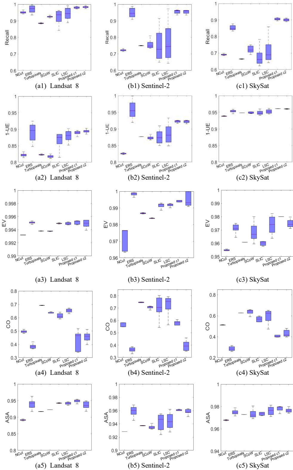
Fig.11. Quantitative evaluation boxplot of the superpixel segmentation results of Landsat 8, Sentinel-2, and SkySat. (a1)-(c1) Recall, (a2)-(c2) 1-UE, (a3)-(c3) EV, (a4)-(c4) CO, (a5)-(c5) ASA.
