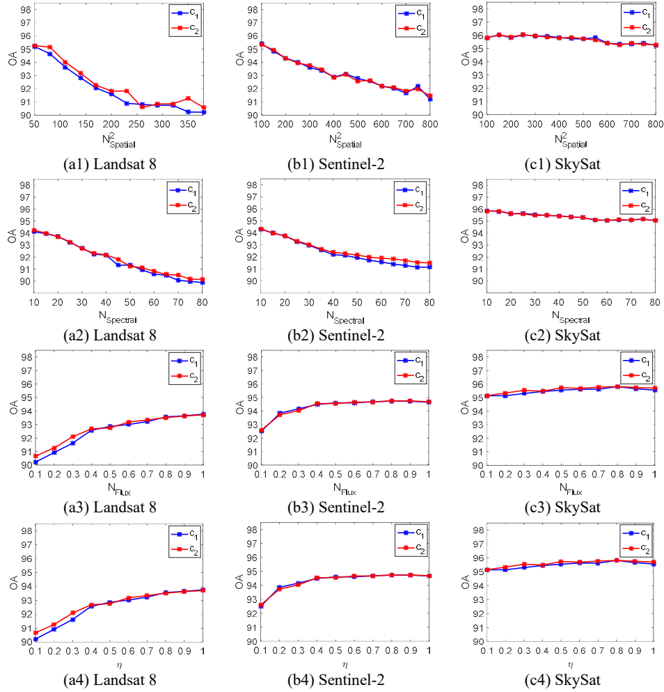
Fig.19. Classification accuracy changing with parameters. (a1)-(c1) The N_{Spatial} of Landsat 8, Sentinel-2, and SkySat, (a2)-(c2) The N_{Spectral} of Landsat 8, Sentinel-2, and SkySat, (a3)-(c3) The N_{Flux} of Landsat 8, Sentinel-2, and SkySat, (a4)-(c4) the \eta of Landsat 8, Sentinel-2, and SkySat.
