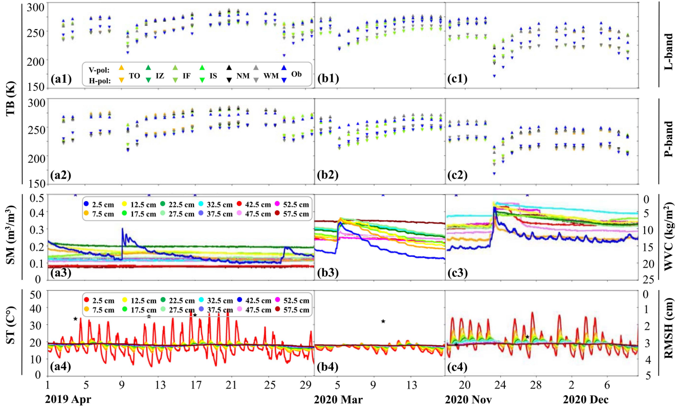
Fig. 3. Observed and estimated brightness temperature using passive microwave models during three bare soil periods: (a) April 2019, (b) March 2020, and (c) November–December 2020, together with associated soil moisture and temperature observations at different soil depths. The blue stars in the soil moisture profile plots represents VWC (in \text{kg/m}^2 ) and the black stars in the soil temperature profile plots represents the RMSH (in cm). The indices 1, 2, 3, and 4 in each figure represent the L-band observation, P-band observation, soil moisture profile, and soil temperature profile, respectively. Note that TO, IZ, IF, IS, NM, and WM refer to the tau-omega, zero-order incoherent, first-order incoherent, incoherent solution, Njoku model, and Wilheit model, respectively.
