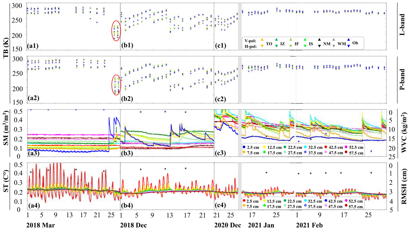
Fig. 4. As for Fig. 3 but under three periods of vegetated soil: (a) grass (March 2018), (b) wheat (December 2018), and (c) corn (December 2020 to March 2021). The blue stars in the soil moisture profile plots represents VWC (in kg/m 2 ) and the black stars in the soil temperature profile plots represents the RMSH (in cm). The indices 1, 2, 3, and 4 in each figure represent the L-band observation, P-band observation, soil moisture profile, and soil temperature profile, respectively. Note that TO, IZ, IF, IS, NM, and WM refer to the tau-omega, zero-order incoherent, first-order incoherent, incoherent solution, Njoku model, and Wilheit model, respectively. The gray area in the corn period is a 17-day gap where the tower was lowered due to unscheduled maintenance.
