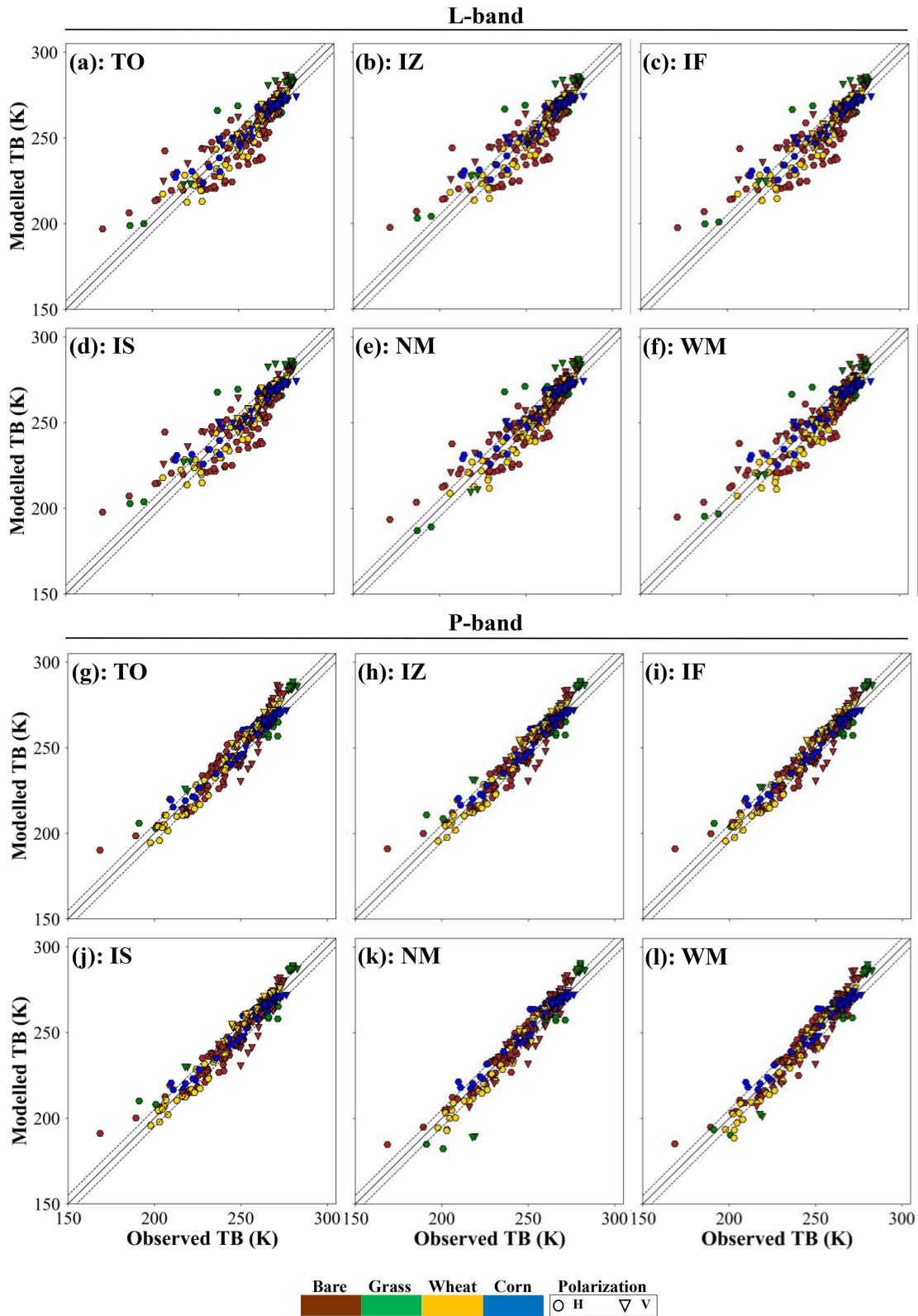
Fig. 6. Scatter plot of the observed and estimated brightness temperature at L-band and P-band using the following models: (a) and (g) incoherent tau-omega (TO), (b) and (h) incoherent zero-order (IZ), (c) and (i) incoherent first-order (IF), (d) and (j) incoherent solution (IS), (e) and (k) Njoku model (NM), and (f) and (l) Wilheit model (WM). The solid line is line 1:1 and the dash lines denote \pm 5 K offset.
