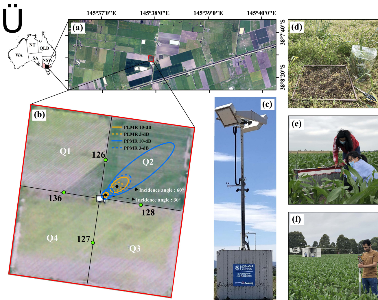
Fig. 1. (a) Location map of (b) experimental site having (c) tower at the center of a paddock at Cora Lynn, VIC, Australia. The colored ovals represent the 3 and 10 dB footprints of the microwave radiometers at incidence angles of 30^\circ and 60^\circ . The green dots on (b) represent the stations installed at the borders of the quadrants Q1–Q4. The ancillary data of (d) VWC, (e) surface roughness, and near-surface soil moisture for 0–5 cm using (f) HDAS, were collected weekly.
