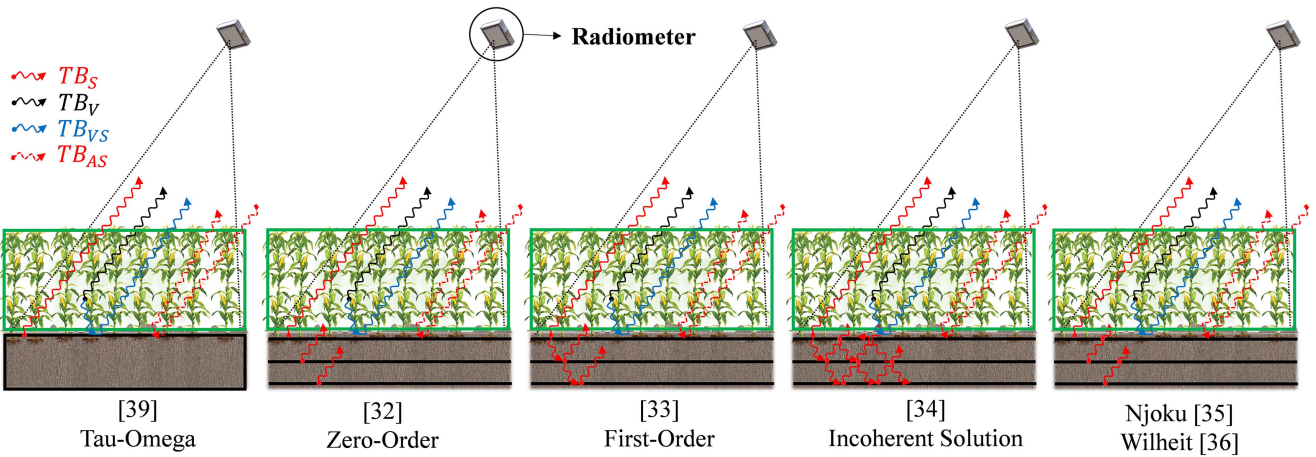
Fig. 2. Schematic of passive microwave emission models. The calculated brightness temperature (TB) for each model includes the sum of TB_S , TB_V , TB_{VS} , and TB_{AS} . TB_S and TB_V represent emissions directly from soil and vegetation, respectively. TB_{VS} is the emission from the vegetation, reflected by the soil, while TB_{AS} is the downward emission from the sky reflected by the soil. Please note that the multilayer incoherent zero-order model and multilayer coherent Njoku and Wilheit models have similar schemes here; however, the former is different from the latter two models in terms of the physics law behind them. In addition, the Njoku and Wilheit models are entirely different in terms of formulation.
