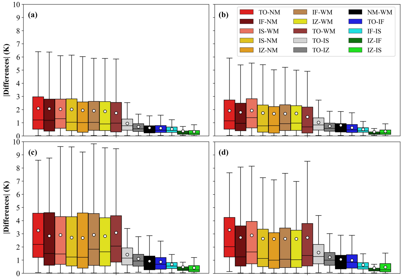
Fig. 5. Absolute difference between pairs of coherent models, incoherent models, and coherent and incoherent models, in terms of their estimation of brightness temperature using (a) L-band (H-polarization), (b) L-band (V-polarization), (c) P-band (H-polarization), and (d) P-band (V-polarization). Please note that TO, IZ, IF, IS, NM, and WM refer to the tau-omega, zero-order incoherent, first-order incoherent, incoherent solution, Njoku model, and Wilheit model, respectively. The white dot in each box represents the average value. The outlier was not shown in the plot due to its high values, suppressing the visualization of boxes.
