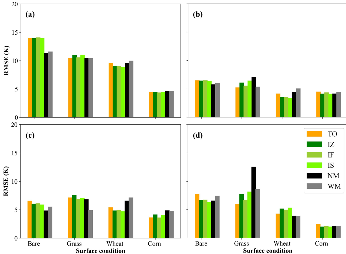
Fig. 7. RMSE between the observed and the estimated brightness temperature at (a) L-band (H-polarization), (b) L-band (V-polarization), (c) P-band (H-polarization), and (d) P-band (V-polarization) for the six different models tested on the four different surface conditions. The abbreviation of the models is interpreted as in Fig. 5.
