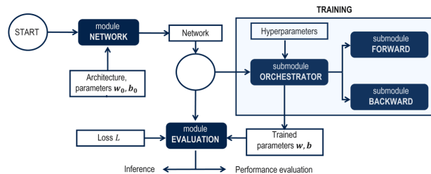
Fig. 1: Proposed framework for HAR personalization.
