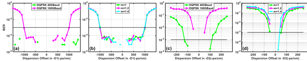
Fig. 9. (a) The influence of dispersion offset in -D1 (relative to optimum value) on BER when transmitting DQPSK signals with different baud rates; (b) The influence of dispersion offset in -D1 on BER with different PM modulation index when transmitting DQPSK signals with 100 Gbaud; (c) The influence of dispersion offset in -D2 (relative to optimum value) on BER when transmitting DQPSK signals with different baud rates; (d) The influence of dispersion offset in -D2 on BER with different PM modulation indexes when transmitting DQPSK signals with 100 Gbaud.
