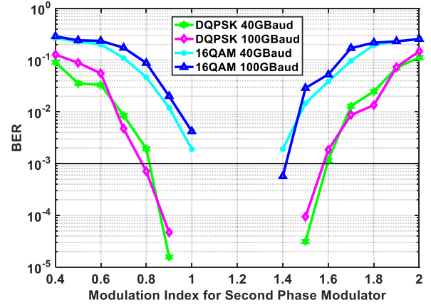
Fig. 11. The influence of modulation index offset between encryption and decryption PMs on BER performance when the data signals have different modulation format and baud rates.
