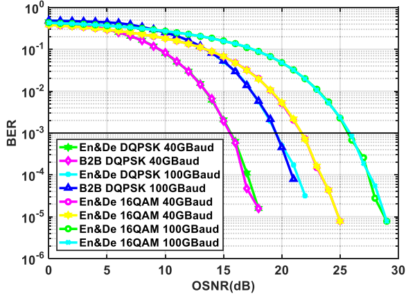
Fig. 7. BER performances of a 50 km secure optical system and the optical back-to-back system without encryption and decryption elements for different modulation formats and signal transmission baud rates.
