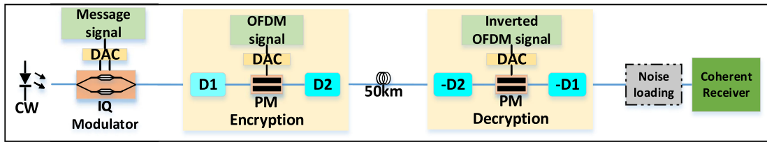
Fig. 1. Physical layer secure coherent optical communication system.
