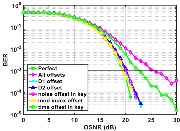
Fig. 12. The influence of adding different offsets in system separately and together on BER performances for DQPSK with 100 GBaud.
