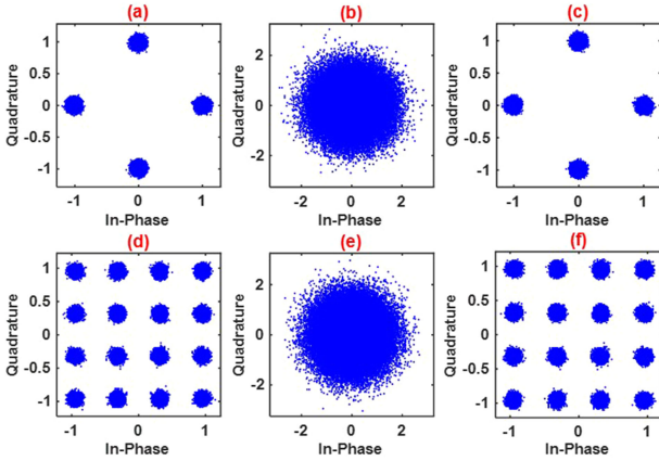
Fig. 3. Transmitted signals are DQPSK and 16QAM at 40 Gbaud, and OSNR is set to 30 dB. (a) DQPSK signal before encryption; (b) Encrypted signal for DQPSK; (c) Decrypted signal for DQPSK; (d) 16QAM signal before encryption; (e) Encrypted signal for 16QAM; (f) Decrypted signal for 16QAM.
