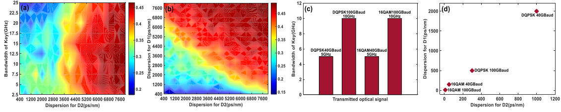
Fig. 2. (a) The influence of bandwidth of security keys on BER for DQPSK signals with 40 Gbaud, fixing D1 to 3000 ps/nm, and determining stable settings for bandwidth of the key; (b) The influence of value of D1 and D2 on BER for DQPSK with 40 Gbaud, fixing bandwidth of key to 5 GHz, and determining suitable values for D1 and D2; (c) Optimum bandwidth of keys for different transmitted message signals under different suitable D1 and D2 values to reach BER = 0.3; (d) Optimum dispersion values for D1 and D2 for different transmitted signals with a security key bandwidth of 10 GHz to reach BER = 0.3.
