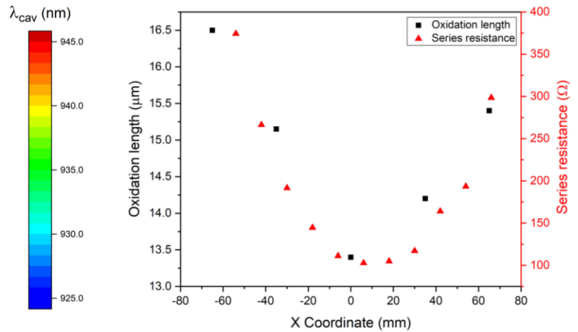
Fig. 10. Radial variation of oxidation length and series resistance measured at 1.8 V for a 38 \mu\text{m} VQF device.
