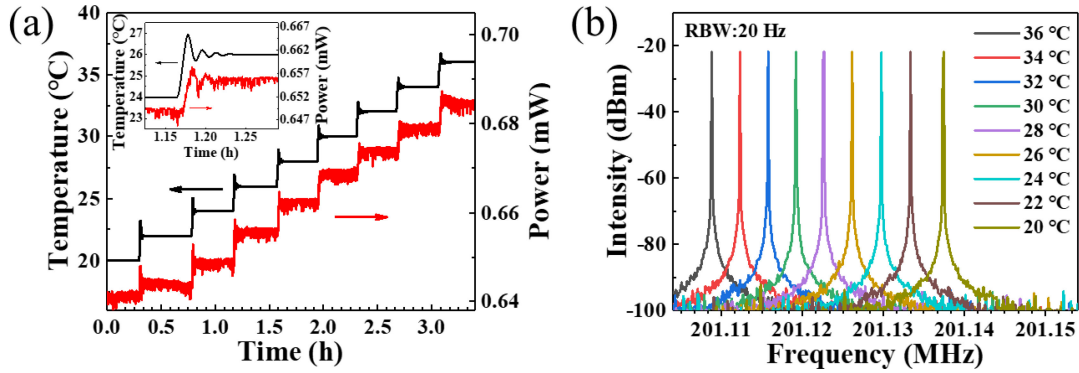
Fig. 3. During thermal tuning (a) the change of output optical power (b) the change of repetition frequency. The inset shows a zoom-in plot of the change from 24 to 26 °C.
