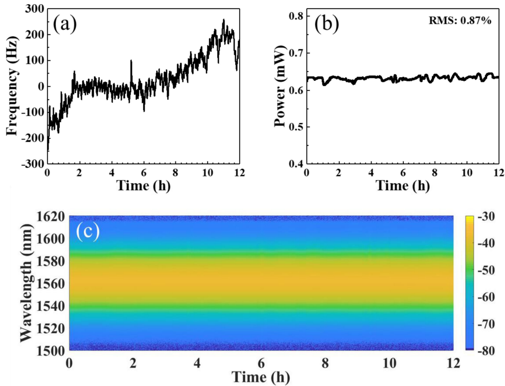
Fig. 4. 12-h measurement of the output show, showing (a) pulse repetition rate, (b) monitored optical power (1/4 of the output power), and (c) optical spectrum, where color bar represents the relative spectrum intensity in units of dBm.
