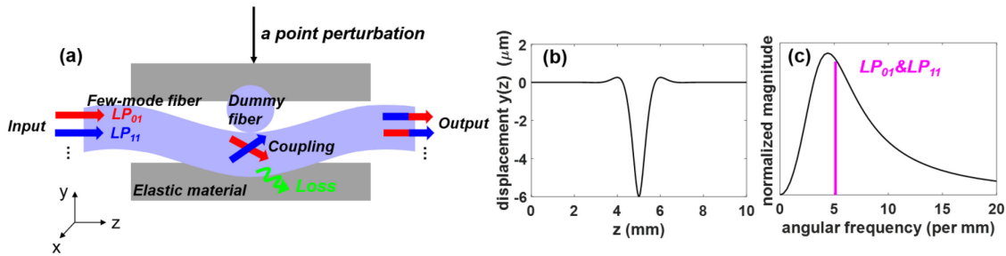
Fig. 1. (a) Schematic of a point-load mode scrambler for few-mode fibers. (b) Fiber displacement along the y-axis under 10 N load and (c) curvature spectrum of a point-load mode scrambler as a function of angular frequency.
