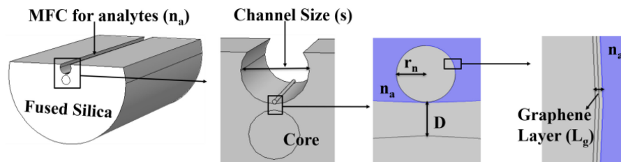
Fig. 1. Cross sectional view of designed sensor.
