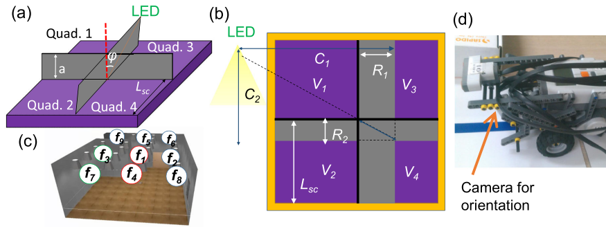
Fig. 1. (a) Principle of QSC for angular diversity AOA VLP Rx. (b) Top view of the QSC with different shadows produced by the barriers. (c) Unit cells with different beacon frequencies for whole area positioning. (d) One example of installing QSC on a robotic trolley.
