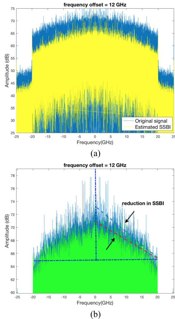
Fig. 10. Electrical spectrum of (a) signal plus SSBI noise (blue/dark) and isolated SSBI (yellow/light colored), and (b) signal plus SSBI noise (blue/dark) and signal with suppressed SSBI (green/light colored).
