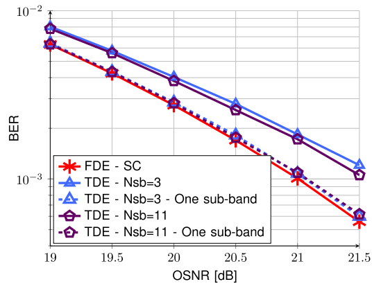
Fig. 4. SC and MSB performances with noise loading; solid line with stars: SC system using FDE; solid lines: MSB system using TDE with 3 (triangles) and 11 (pentagons) sub-bands; dashed lines: MSB system using TDE where one sub-band is simulated at a time for 3 (triangles) and 11 (pentagons) sub-bands, respectively.
