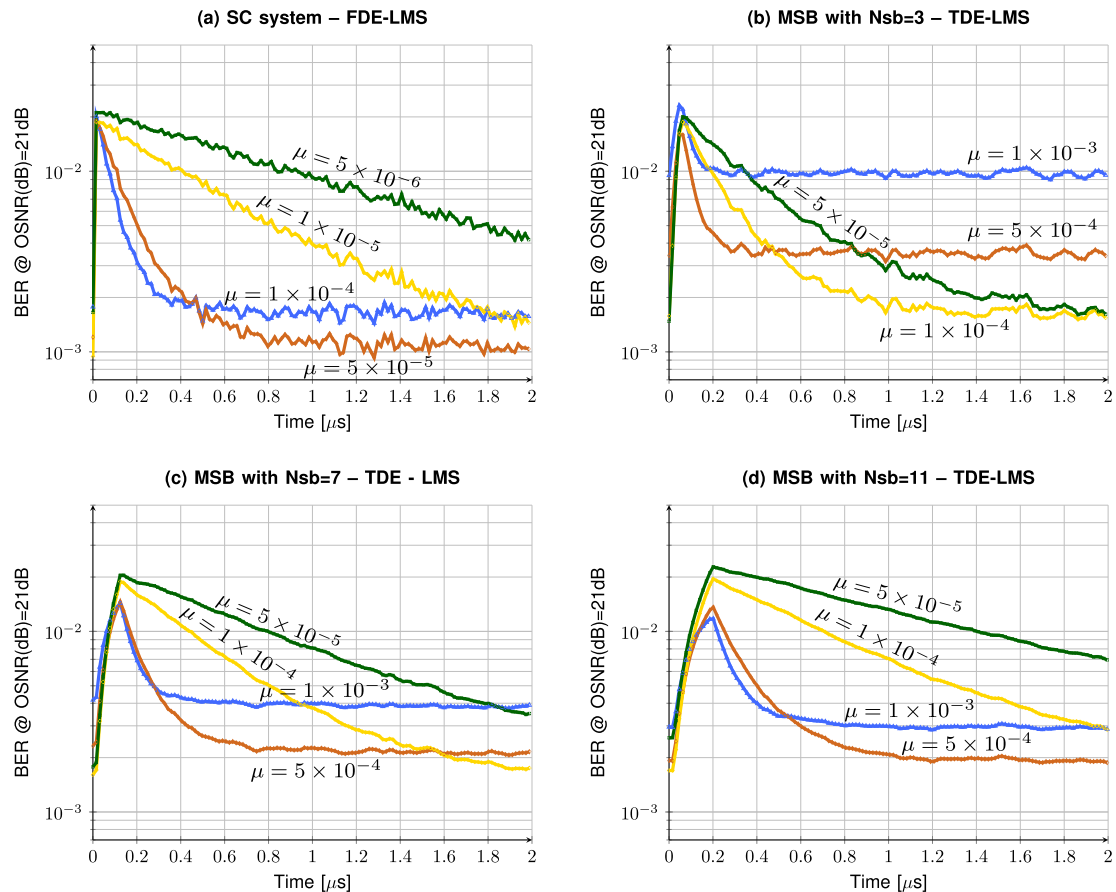
Fig. 7. (a) Convergence performance after perturbation of the SC system using FDE-LMS with different step sizes. (b)–(d) Convergence performance after perturbation of a MSB system with 3, 7 and 11 sub-bands using TDE-LMS with different step sizes. The simulated channel includes -30 dB/km crosstalk, 20 ps/km DMD. The CD is fully compensated by static equalizers. The resolution in time is 0.015 \mu s.
