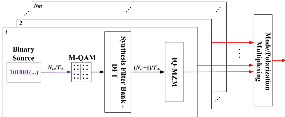
Fig. 1. MSB transmitter architecture.
