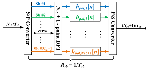
Fig. 2. Synthesis filter bank architecture.
