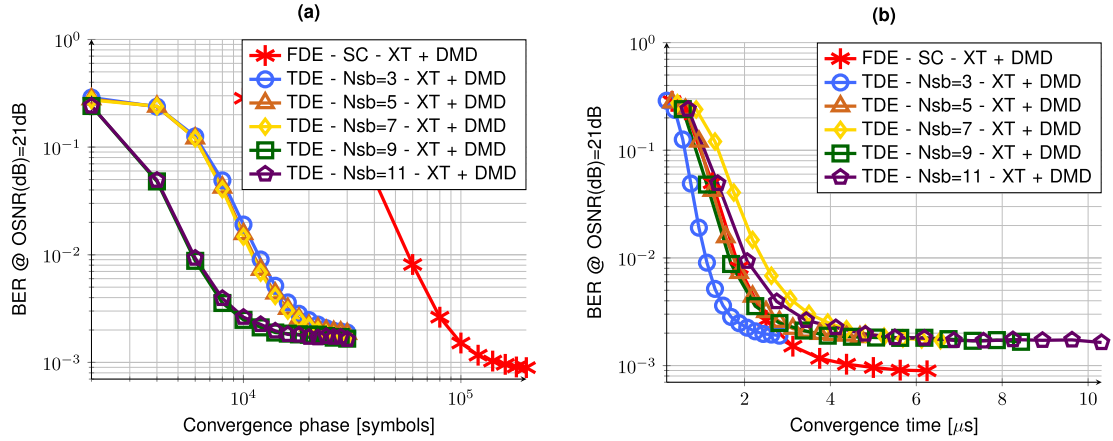
Fig. 6. Convergence period for OSNR = 21 dB of MSB and SC systems with -30 dB/km crosstalk and 20 ps/km DMD; (a) in number of symbols, and (b) in microseconds. Stars: SC system using FDE. Remaining symbols: MSB system for 3 (circles), 5 (triangles), 7 (diamonds), 9 (squares) and 11 (pentagons) sub-bands using TDE.
