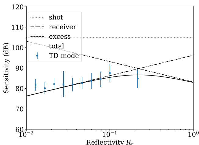
Fig. 8. The measured and modeled sensitivity characteristics for a single detector TD-OCT signal.
