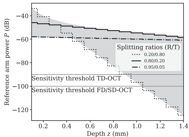
Fig. 2. The reference arm power of MR-OCT was calculated based on the SLED power of 13 mW with a PM splitting ratio of R/T = 80/20 (solid bold line) and OD 1.0 attenuation. The gray area represents the possible powers that can be achieved through the selection of other splitting ratios. The boundaries are plotted for ratios R/T = 20/80 and 95/5 (dotted and dot-dash respectively). Two guides for assumed sensitivity levels of 100 dB [19] and 90 dB [24] are shown.
