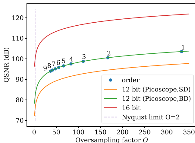
Fig. 7. Digitizer QSNR limitation vs. oversampling factor vs. order of reflection. Due to oversampling the signal SNR can improve somewhat due to averaging effects according to bit_+ = \log(O)/\log(4) where O is the oversampling factor [40]. The position of nine orders of reflections are indicated for the balanced detection limit (12 bit (Picoscope, BD)).
