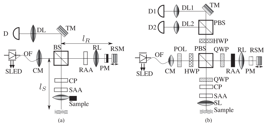
Fig. 6. Two configurations of MR-OCT were used; namely (a) single detection MR-OCT and (b) balanced detection MR-OCT. The components used included SLED: superluminescent diode, OF: optical fiber, CM: collimator lens, BS: non-polarizing beam splitter, PBS: polarizing BS, CP: compensator plate, TM: turning mirror, DL: detector lens, D: detector, SL: sample arm lens, RL: reference arm lens, SRM: reference axially scanning mirror, PM: partial mirror, (S/R)AA: sample/reference arm attenuator, POL: polarizer, HWP: half wave plate, QWP: quarter wave plate.
