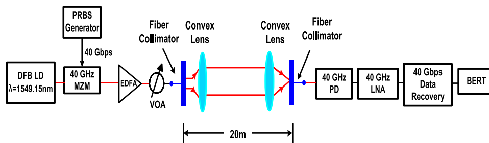
Fig. 1. Experimental configuration of the proposed 20 m/40 Gb/s FSO links which employ a 1550-nm externally modulated laser transmitter cascaded with an EDFA and a pair of fiber collimators.
