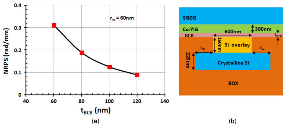
Fig. 3. (a) NRPS as a function of BCB thickness ( t_{BCB} ). (b) Waveguide cross-section of nonreciprocal phase shifter.
