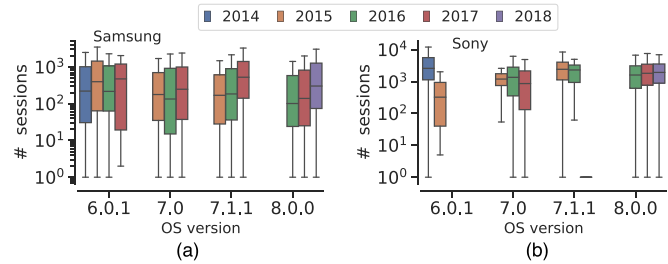
Fig. 12. Number of sessions created by user per Android OS version for Samsung and Sony mobile phones. The color shows the year of release of the devices to the market. Users with recent device models have created more number of sessions.
