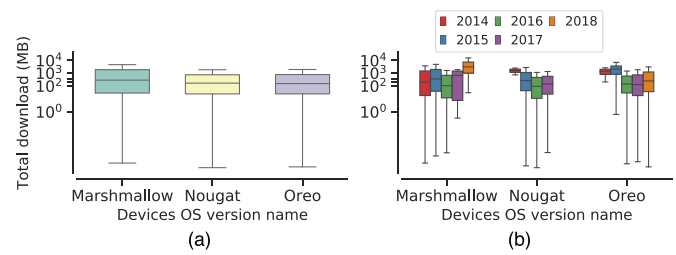
Fig. 13. Total downloaded bytes per user categorized by Android OS version and year of release of the devices (LTE network). New devices with the latest Android OS have relatively less total downloaded bytes than similar device models (based on year of release) but with older OS version.
