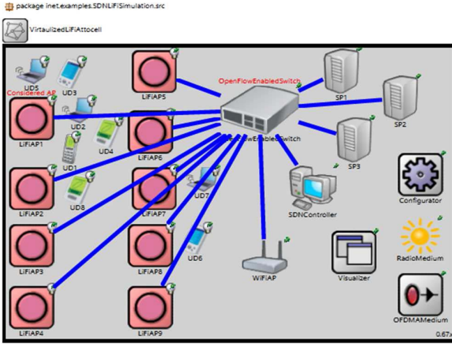
Fig. 7. Virtualized LiFi attocell access network simulation environment in OMNeT++.
