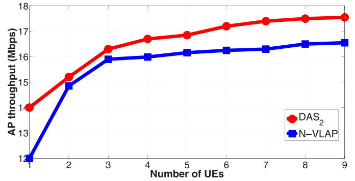
Fig. 15. Throughput comparison of DAS 2 to N-VLAP.
