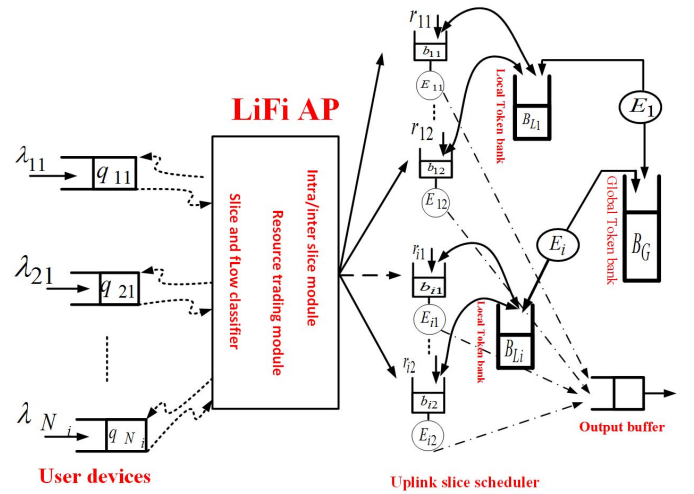
Fig. 5. LiFi Uplink slice scheduler.
