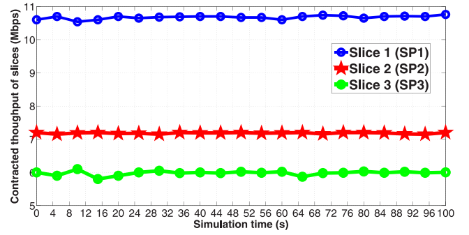
Fig. 9. Fixed throughput for slices ( S_1 (45%), S_2 (30%), S_3 (25%).).
