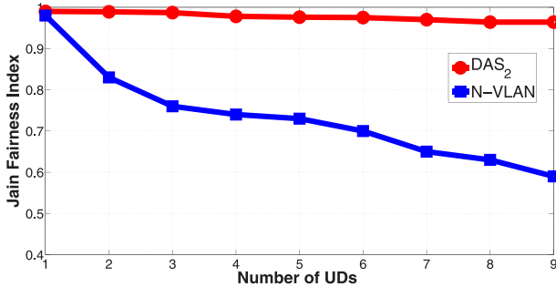
Fig. 14. Airtime fairness comparison of DAS 2 to N-VLAP.
