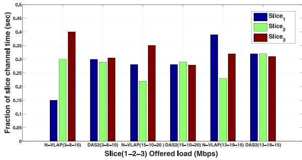
Fig. 13. Fractional of slice channel time under varying offered traffic load.
