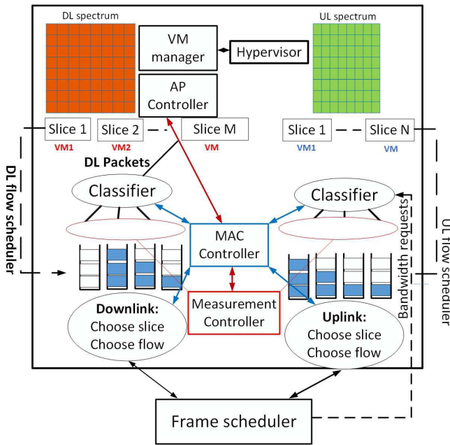
Fig. 2. A modified basic design of LiFi AP attocell virtualization [14].
