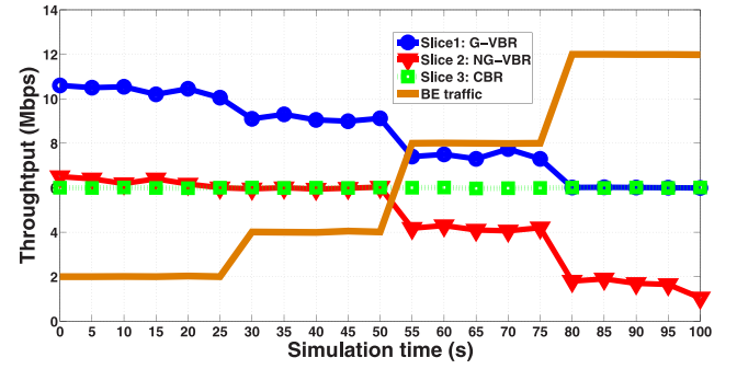
Fig. 10. Throughput of slices under different BE traffic loads.
