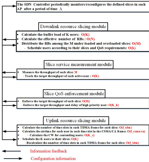
Fig. 6. Resource slicing scheme pseudocode.
