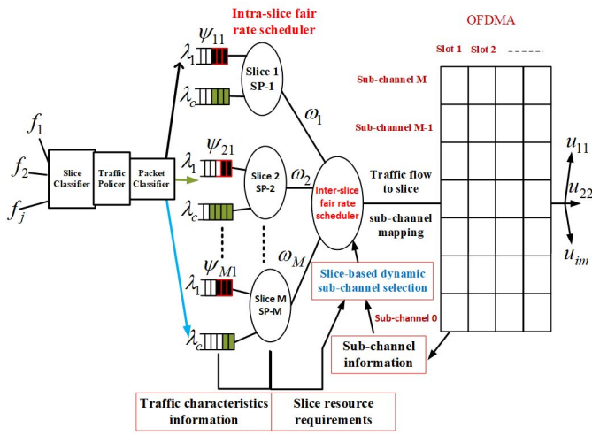
Fig. 4. LiFi Downlink spectrum virtualization.
