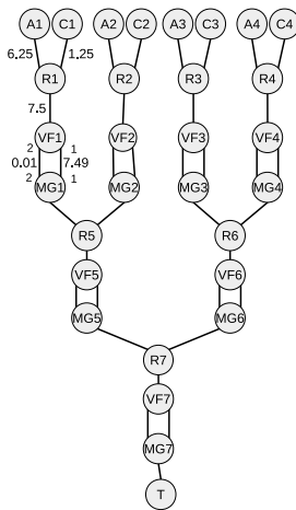
Fig. 10. Evaluation topology N2.
