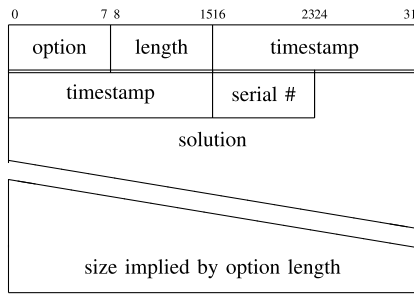
Fig. 6. Proof-of-work as IP option.
