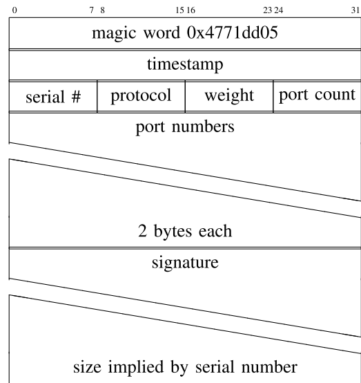
Fig. 5. Flow cookie as ICMP Echo payload.
