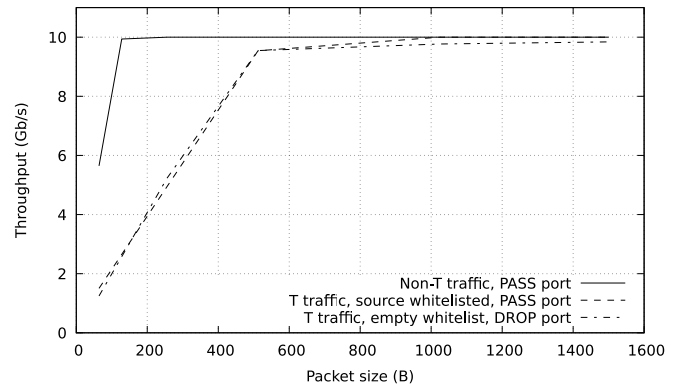
Fig. 14. Throughput in Experiment 4.
