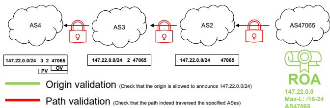
Figure 1. Origin validation binds resources to ASNs. Path validation ensures that an announcement took the path contained in the BGP AS path attribute. Path validation requires origin validation to work properly.
