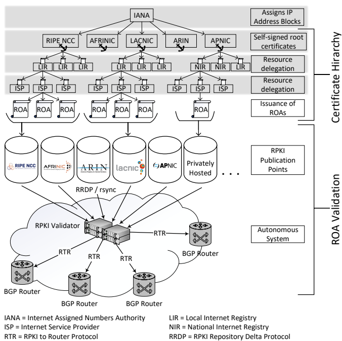
Figure 2. RPKI architecture: The IANA delegates resources to the five RIRs, each of which maintains a trust anchor. They continue to delegate smaller chunks of the resources to their subordinates. An ISP at the end of the chain will create a ROA which is published at a publication point. RPKI validators fetch from the publication points via RRDP or rsync to cryptographically validate the data and send the resulting file via the RTR protocol to the BGP routers for inclusion in the BGP route selection process.
