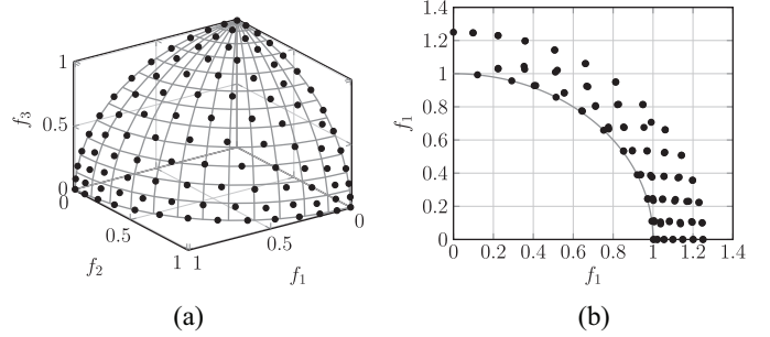
Fig. 2. Comparison of population distributions when decreasing the number of objectives on DTLZ2. (a) Approximation in the 3-D case. (b) After decreasing one objective.
