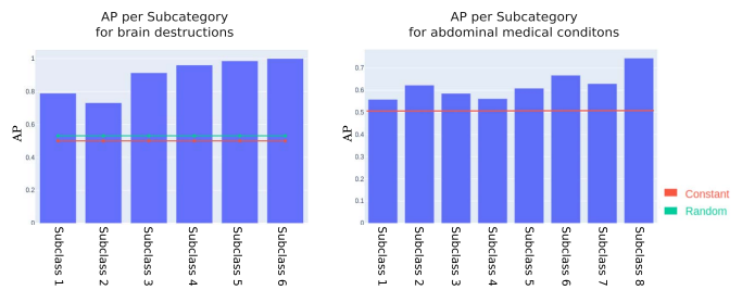
Fig. 6. Median submission performance on sub-classes of two different anomaly categories. The sub classes (classes 1-6, 1-8) are sorted by human perceived difficulty in descending order, i.e. class 1 is the class which was perceived as the hardest and classes 6 (and 8) are the classes perceived as being easiest.
