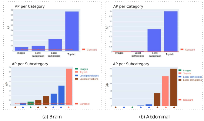
Fig. 8. Pixel-level AP for the different anomaly categories. The top row shows the mean of the grouped categories, and the second row gives more detailed results of subcategories, i.e. the top row categories split up in fine-grained subcategories. Median submission performance was used as the basis for the subcategories.
