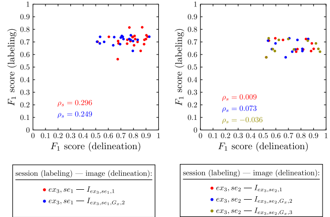
Fig. 8. Scatterplot of individuals' F_1 scores for ROI labeling and ROI delineation in experiment 3, session 1 (left) and session 2 (right). Spearman's rank correlation coefficient given as \rho_s . G_X : result data combined from G_1 and G_2 .
