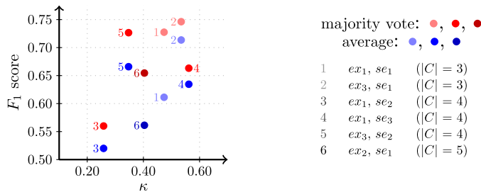
Fig. 1. Overall F_1 scores in relation to Fleiss' \kappa for inter-annotator agreement (ROI labeling). Shown are the average (blue) and majority vote (red) in the different experiments ( ex_1, ex_2, ex_3 ) and sessions ( se_1, se_2, se_3 ). The darker the color, the higher the level of complexity indicated by the number of classes |C| . The ids 1–6 are only used to label the dots.
