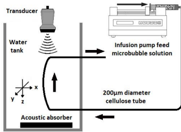
Fig. 1. Illustration of the experimental setup for microbubble localization. The transducer acquired the data from MBs that were located in the parabolic part of the tube in the center of the tank.
