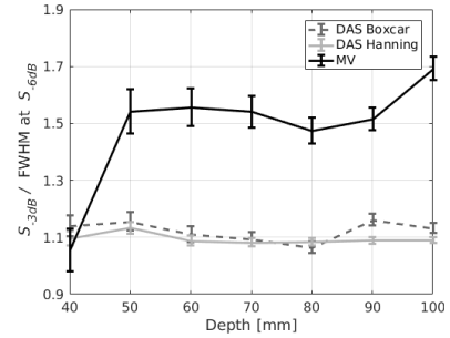
Fig. 12. Critical separation limit ( S_{-3dB} ) and FWHM at significant separation limit ( S_{-6dB} ) ratio variation as a function of depth for DAS and MV responses.
