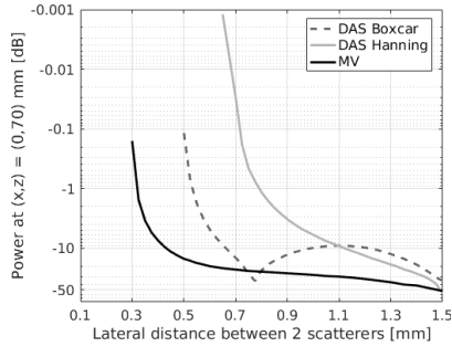
Fig. 4. Variation of maximum power drop between two scatterers at (x, z) = (0, 70) mm as a function of their lateral separation distance. The simulated scatterers were positioned symmetrically around x = 0 .
