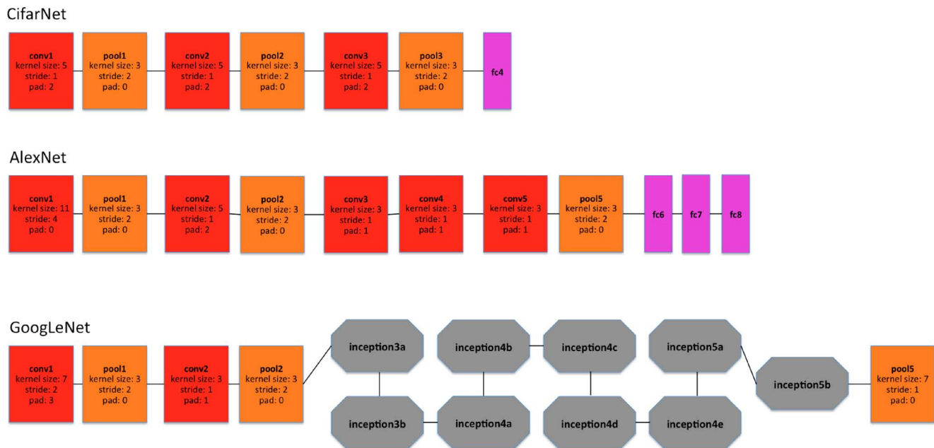
Fig. 5. A simplified illustration of the CNN architectures used. GoogLeNet [33] contains two convolution layers, three pooling layers, and nine inception layers. Each of the inception layer of GoogLeNet consists of six convolution layers and one pooling layer.
