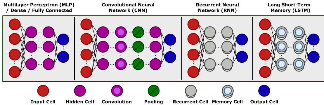
Fig. 2. Popular Artificial Neural Network (ANN) structures. MLP/Dense/Fully Connected are typically well-suited for cross-sectional quantitative data, whereas Recurrent Neural Networks (RNNs) and Long Short Term Memorys (LSTMs) networks are optimized for sequential data. Convolutional Neural Networks (CNNs) are equipped for both types.
