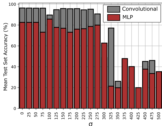
Fig. 8. Simulation results investigating the performance of MDNNs for hand gesture classification adopting non-ideal Pt/Hf/Ti ReRAM devices. Device-to-device variability is simulated using MemTorch [108].
