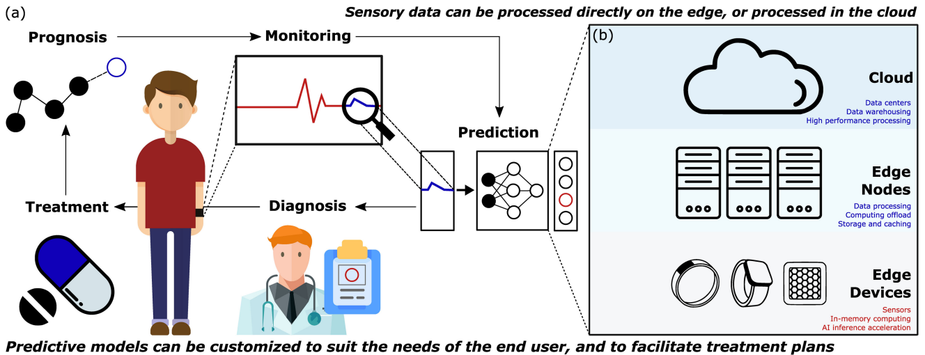
Fig. 1. Depiction of (a) the usage of DL in a smart healthcare setting, which typically involves monitoring, prediction, diagnosis, treatment, and prognosis. The various parts of the DL-based healthcare system can run on (b) the three levels of the IoT, i.e. edge devices, edge nodes, and the cloud. However, for healthcare IoT and PoC processing, edge learning and inference is preferred.
