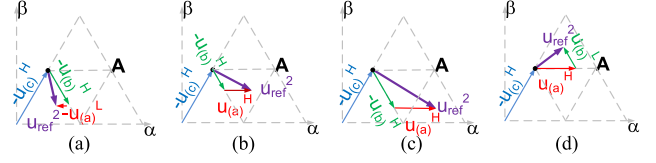
Fig. 8. Generating a reference voltage vector U_{\text{ref}} located in individual subsectors of sector A (a)–(d) using method 3. The reference voltage vector U_{\text{ref}2} components are determined as (11).
