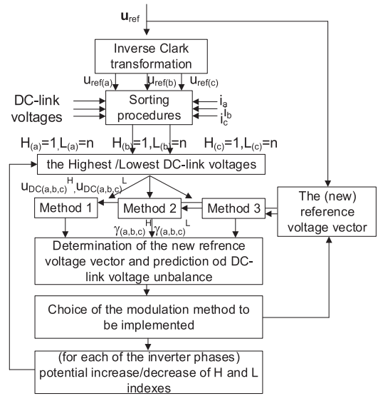
Fig. 9. Diagram of the proposed SVPWM method.
