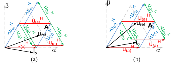
Fig. 3. Preselected active vectors for the case of unbalanced dc-link voltages and the reference voltage vector position (a) \alpha_u = \pi/9 and (b) \alpha_u = 2\pi/9 . The output current vector position \alpha_i = \alpha_u - \pi/6 . Indexes: “H” – the H-bridge with highest dc-link voltage, “L” – H-bridge with the lowest dc-link voltage, (-) denotes negative H-bridge output voltage.
