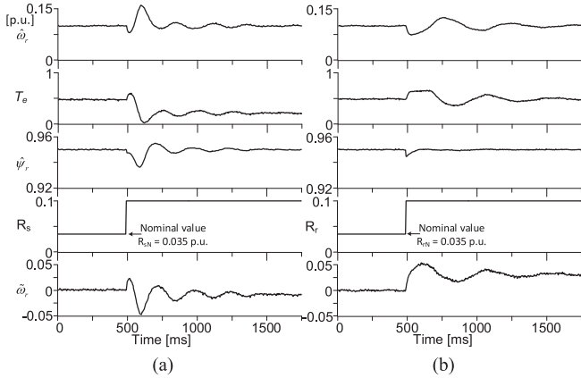
Fig. 15. a) After 500 ms the nominal value of stator resistance is changed up to 0.1 p.u., the rotor speed is reproduced nonadaptively (48), the machine is loaded about 0.5 p.u.
