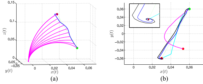
Fig. 5. (a) Performance of the designed fuzzy controller used to track a straight line trajectory (Unit: m). The trajectory of the continuum manipulator tip in 3-D task space are captured and illustrated in blue line and the central backbone shape of the continuum manipulator is illustrated in pink. The green dot indicates the initial position [0.06, 0.06, 0.03]^T and the red dot indicates termination position [0.03, -0.06, 0.135]^T . The green-dotted line shows the specified reference trajectory. (b) Performance comparisons of the four controllers shown via the xy plane view of 3-D task space. The blue, black, cyan, and pink trajectories indicate the trajectories based on the controllers “I-A,” “I-B,” “I-C,” “I-D,” respectively. A “zoom-in” view around the target is presented, which shows the spiral phenomenon associated to our fuzzy controllers.
