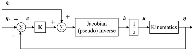
Fig. 6. Overview of a closed-loop control that is based on the (pseudo) inverse Jacobian method. Control input includes both the desired time-varying task trajectory and the preplanned task space velocity with respect to the desired task (trajectory) [15], [34]. \mathbf{K} is a diagonal matrix, and if \mathbf{K} = \mathbf{0} , then this control architecture becomes an open-loop control.
