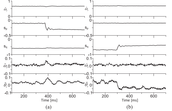
Fig. 10. (a) Reactive power is equal to -0.6 p.u. and after 400 ms, the active power is changed to -0.35 p.u. (b) Active power is -0.1 p.u. and after 300 ms, the reactive power is changed to -0.4 p.u.
