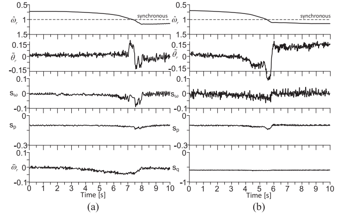
Fig. 11. Characteristic speed observer waveforms for the crossing of generator rotor speed through synchronous speed for (a) value of c_f is determined adaptively from (44), and (b) c_f = 11 and it is constant.
