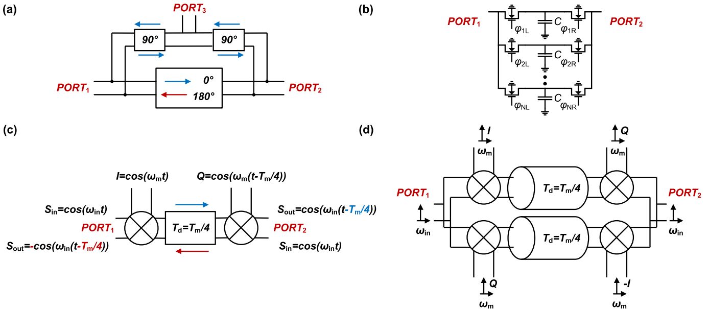
Fig. 2. Block diagram of (a) staggered-commutation circulators, showing (b) N-path filter implementation of the non-reciprocal branch, (c) single-branch, and (d) IQ double-branch implementations of the broadband gyrator.
