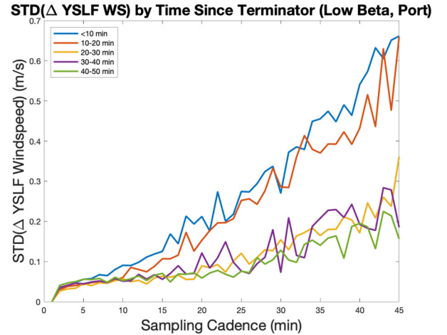
Fig. 7. Standard deviation of YSLF wind-speed error as a function of sampling cadence period at various orbit sectors. The errors due to increased blackbody sampling rates are greatest immediately after crossing the terminator. This effect is largest at longer sampling periods.
