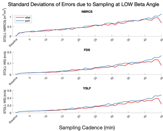
Fig. 4. Standard deviations of growth in error as a function of sampling cadence for (Top) NBRCS, (Middle) FDS wind speed, and (Bottom) YSLF wind speed at low beta angle. Red traces indicate the values for the starboard antenna, and blue traces indicate the values for the port side.
