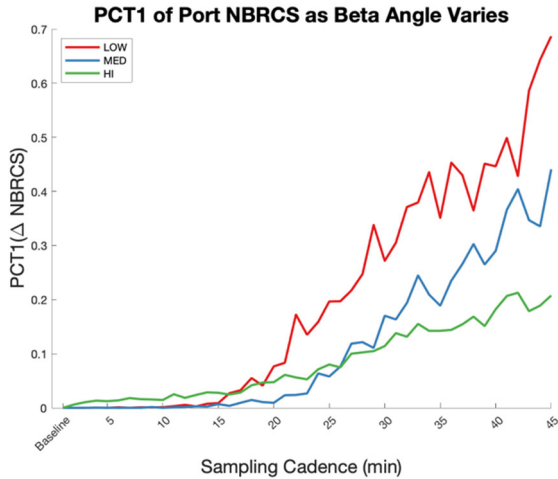
Fig. 6. PCT1 of NBRCS error as a function of sampling cadence period at various beta angles. At lower beta, the performance degradation is more pronounced.
