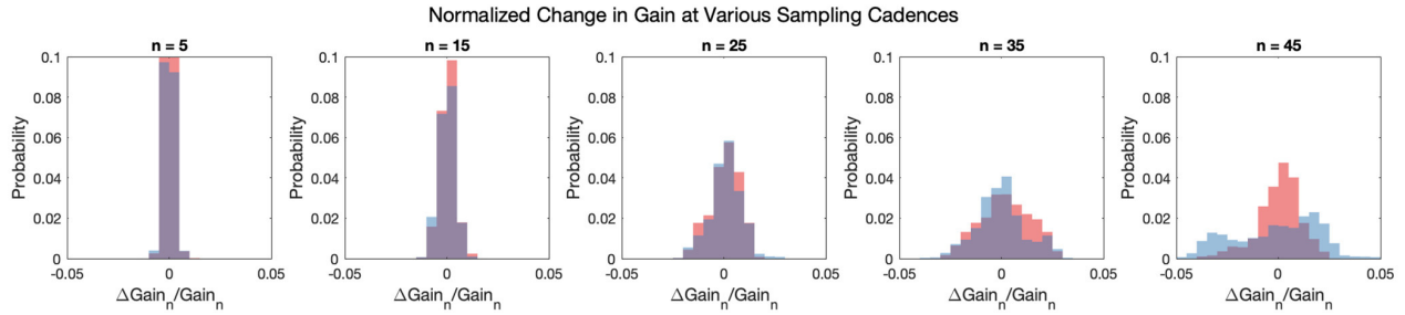
Fig. 3. Histograms of gain error at n = \{5, 15, 25, 35, 45\} min. The blue and red distributions represent data from the port and starboard antennas, respectively. At low n , the gain error approaches a delta function. As sampling cadence time increases, the distribution widens, illustrating the degradation from the original 1-min sampling cadence.
