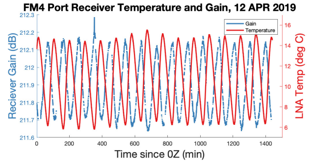
Fig. 1. Example of temperature influence on receiver gain. (Top) FM4's port receiver gain is plotted (blue) with the temperature at a nearby probe (red) for a full day starting at 0Z 12 APR 2019. Note that gain is inversely related to local temperature and that these swings are periodic, consistent with CYGNSS's 95-min orbital period.
