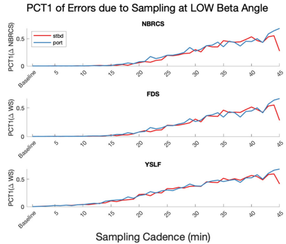
Fig. 5. PCT1 of error as a function of sampling cadence period for (Top) NBRCS, (Middle) FDS wind speed, and (Bottom) YSLF wind speed at low beta angle. Red traces indicate values for the starboard antenna, and blue traces indicate values for the port side.
