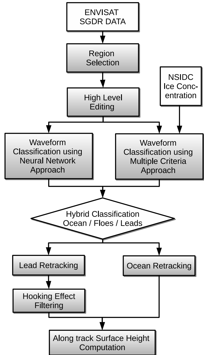
Fig. 3. Flowchart describing the data processing for the along track SSH computation in the Arctic Ocean
