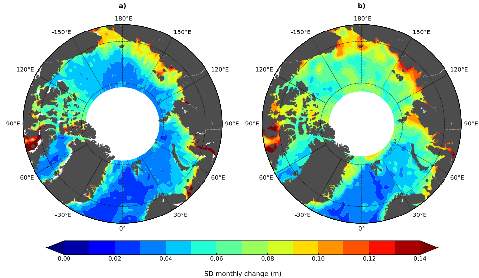
Fig. 17. Standard deviation of monthly change in the Arctic SLA from June 2002 to May 2010. (a) Computed for the new solution. (b) Computed with DTU Arctic SLA maps.
