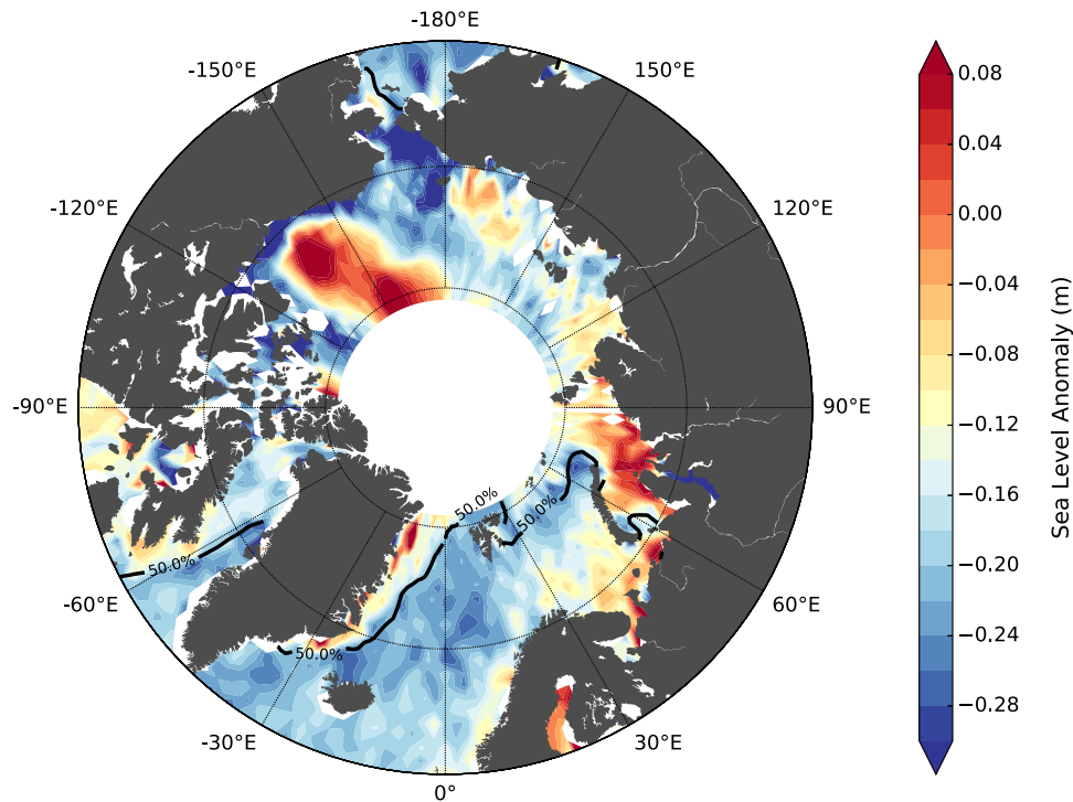
Fig. 16. Gridded map of the Arctic SLA for December 2007 produced by the new retracking solution (box 2^\circ \times 1^\circ ). The solid dark curve is the contour of 50% SIC (from OSI-SAF) for the same month.
