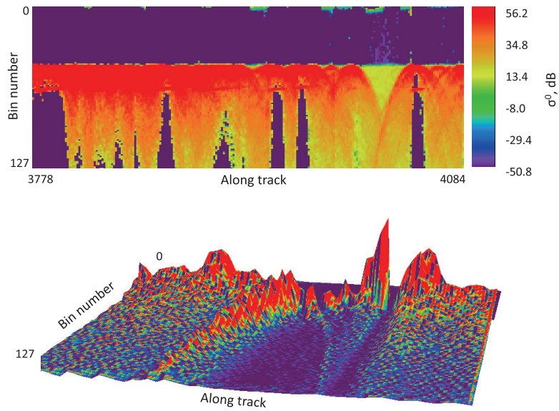
Fig. 12. Example of hooking where leading edge follows a hyperbola as altimeter approaches and recedes from a bright specular point. (a) Radargram illustrating power in each waveform bin for a section ~110 km along track (306 waveforms) with the color indicating intensity on a logarithmic scale to show the wide range of values. There is minimal power in bins 0–40 with a steep leading edge around bin 45. Strong reflectors dominate even away from nadir with the delayed responses producing hyperbolae. (b) 3-D representation of the power in each bin for a shorter segment.
