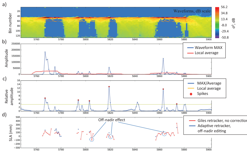
Fig. 13. (a) Series of 370 ENVISAT RA-2 waveforms spanning 120 km along track. (b) Power value in bin at the top of leading edge (absolute units) and the result of a running 21-point mean. (c) Ratio of actual value to 21-point mean, with a threshold for peak detection at 3.5. (d) SLA calculated using the Giles and the adaptive retracker. For the latter, the five waveforms either side of a “significant peak” are discarded, so the rapid spatial changes associated with hooking are avoided.
