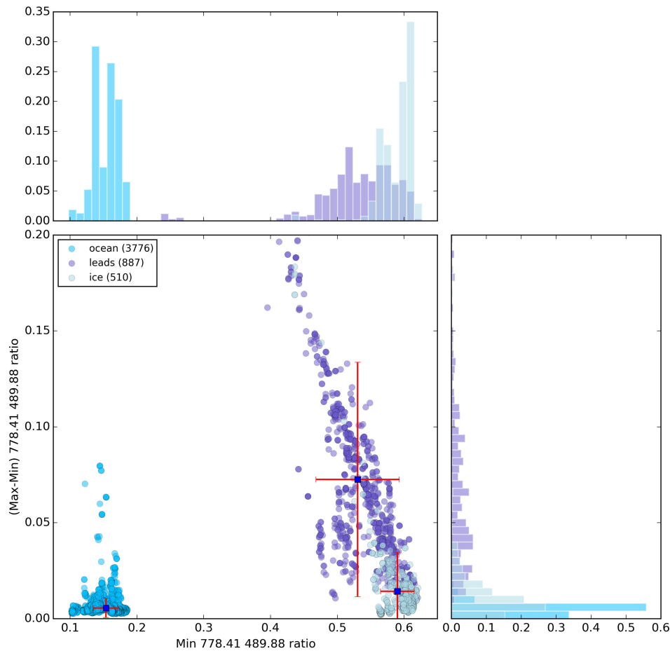
Fig. 8. Variation of normalized radiance ( r_{778}/r_{490} ) within a 7 \times 7 box. (a) and (c) Histograms for the two axes. (b) Scatter plot of minimum value against the difference of the maximum and minimum values with coloring according to the altimeter classification.
