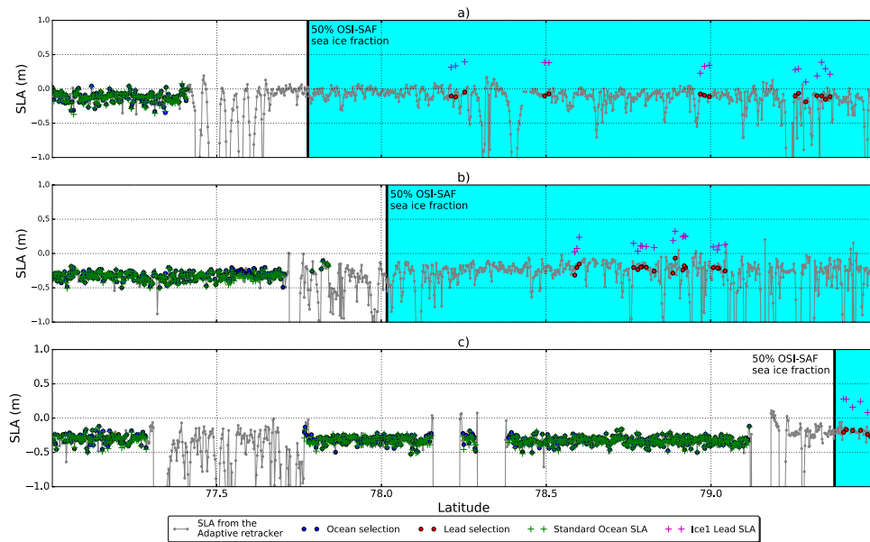
Fig. 15. SLA profiles on ENVISAT pass 788 for (a) cycle 64 (December 2007), (b) cycle 66 (March 2008), and (c) cycle 69 (June 2008), contrasting the performances of different retracker. The SLA computed with the adaptive retracker is plotted in gray curve. Measurements classified as “ocean” are colored in dark blue dots and points classified as “leads” are colored in red dots. Green crosses: SLA computed with the ENVISAT standard ocean retracker on the “ocean” points. Magenta crosses: SLA computed using the ice1 retracker from the ENVISAT products on “leads” points. Only points definitely classified as “ocean” or as “leads” are used in our analysis. The output of the standard ocean retracker lies close to that of the adaptive retracker, whereas, in this instance, the ice1 retracker for leads gives much higher values.
