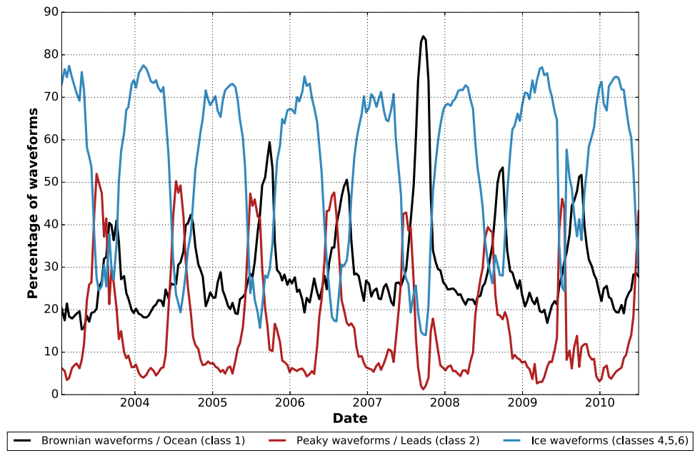
Fig. 5. Temporal evolution of the class proportion identified by the neural network algorithm during the ENVISAT period over the ocean above 60° of latitude.
