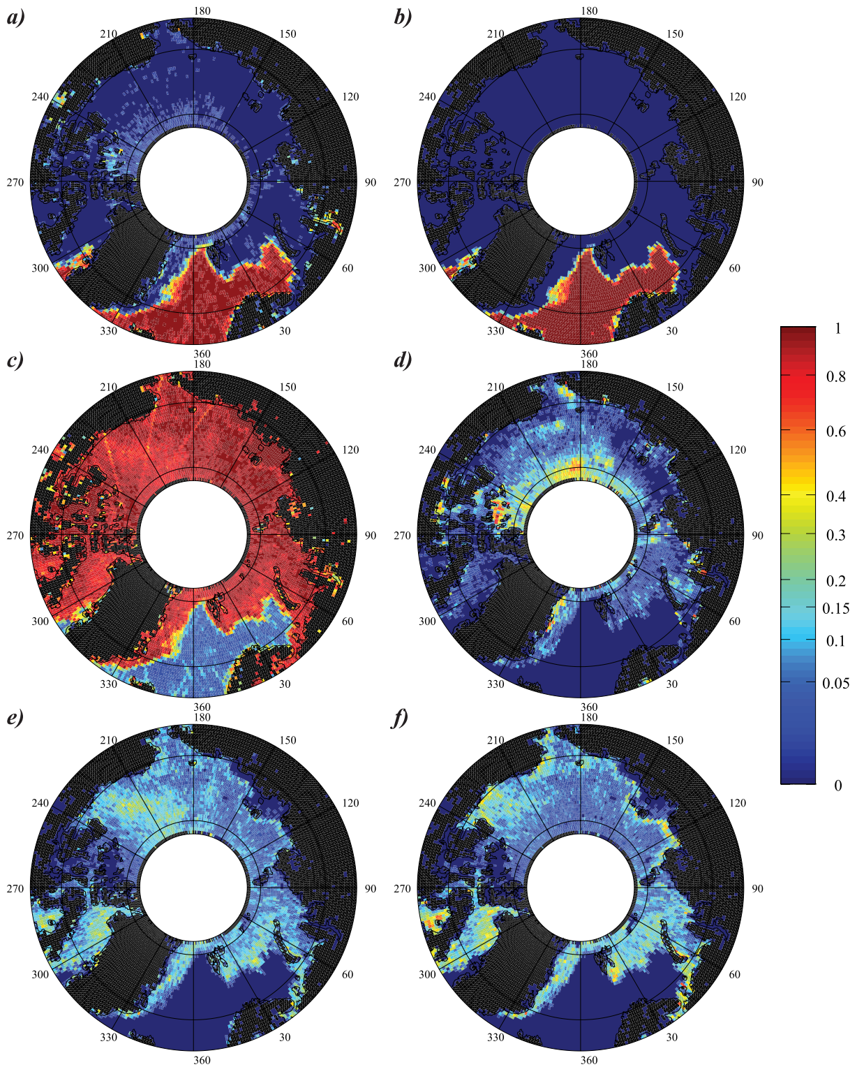
Fig. 4. Comparison of percentages of classifications according to (a), (c), and (e) neural net and (b), (d), and (f) multiple-criteria approach. (Top row) "Ocean" (class 1). (Middle row) "Floes" (classes 4-6). (Bottom row) "Leads" (class 2). Color bar has a nonlinear scale to enhance the differences at low percentages.
