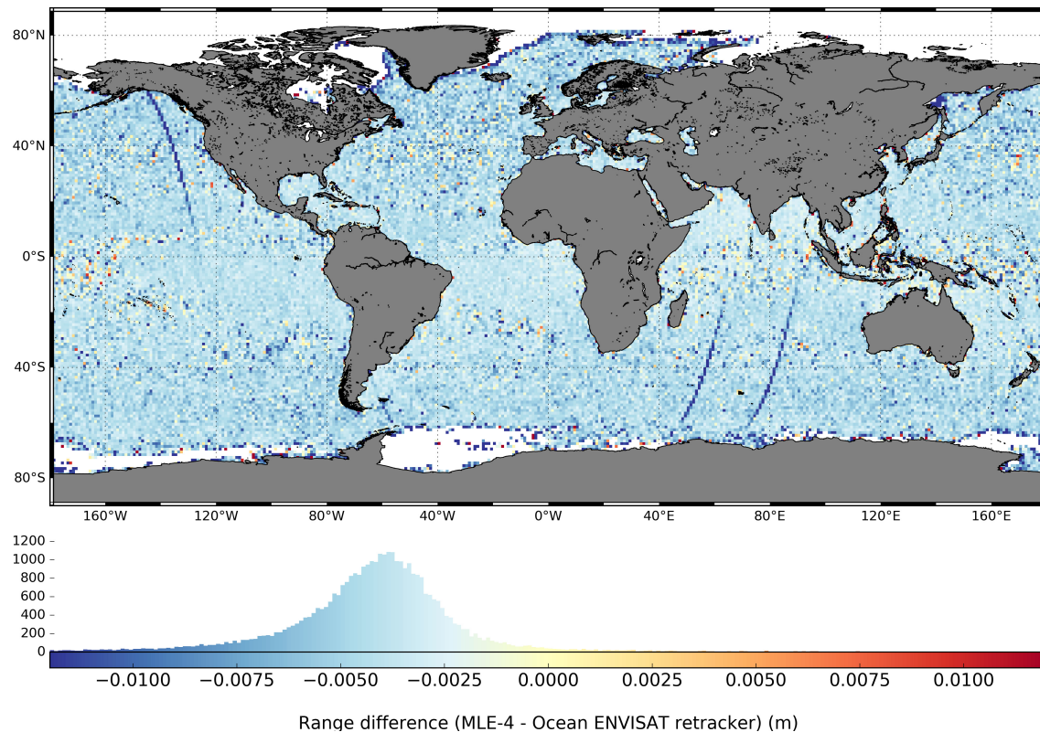
Fig. 14. Gridded map of the range difference between the adaptive retracker and the standard ENVISAT/RA-2 ocean retracker over open ocean on cycle 85 ( 1^\circ \times 1^\circ ). The histogram of the differences is presented at the bottom, which has a mean bias of -6.28 mm and a standard deviation of 2.37 mm.
