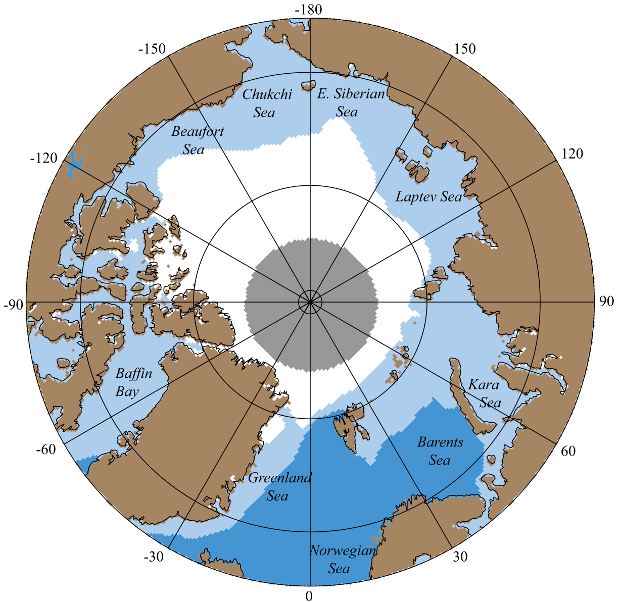
Fig. 1. Map of Arctic Ocean with mean ice extent in September shown in white and the mean ice extension for March in light blue. (Figure derived from 50% SICs for March and September from SSM/I data for 1979–2015, provided by NSIDC. The central gray disk marks region for which there is no SSM/I coverage. Individual years will have greater or less coverage than shown.)
