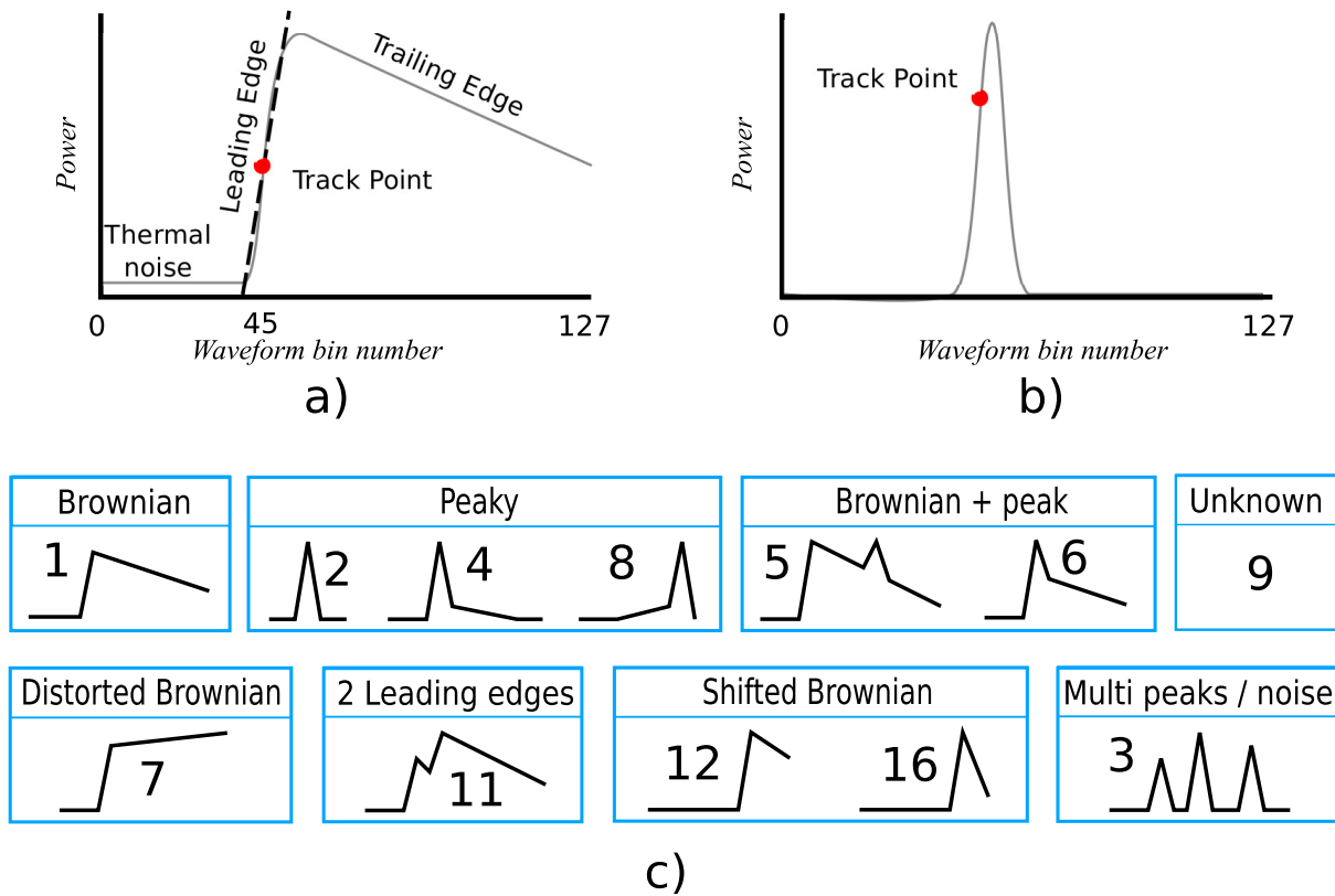
Fig. 2. Illustration of the different Arctic waveform shapes. Schematic of (a) typical ocean (“Brown”) waveform and (b) ice lead waveform, both of which are retracked in this paper. (c) More extensive variety of waveform shapes that may be encountered, and upon which the neural net is trained.
