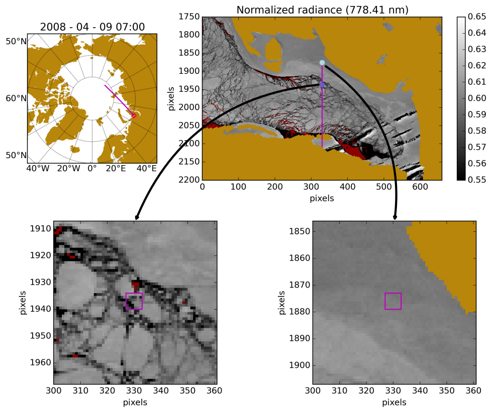
Fig. 6. Example MERIS data for April 9, 2008. (a) Map showing location of swath. (b) Zoomed-in view of region at southern end of track with pink line showing altimeter nadir view, orange indicating land, and red mark indicating cloud. (Note unflagged pixels in the bottom-right corner of image). (c) and (d) Details of regions of leads and ice floe, respectively, showing the greater spatial heterogeneity in the former. Pink box: example regions of 7 × 7 pixels.
