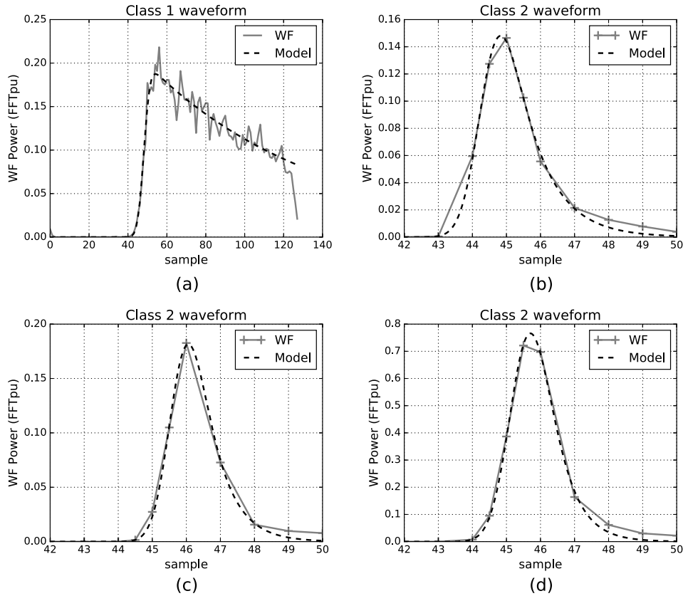
Fig. 10. Retracked modified Brown model superimposed on ENVISAT waveforms over (a) ocean and (b)–(d) three different sea-ice lead waveforms with their associated waveform class assigned by the neural network classification. The two DFT samples added by the RA-2 altimeter are considered and are localized at samples 44.5 and 45.5 (starting from 0).
