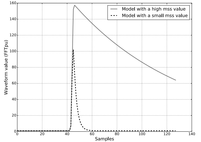
Fig. 11. Modified Brown model with a high mss value (gray solid curve) and a small mss value (black dashed curve)
