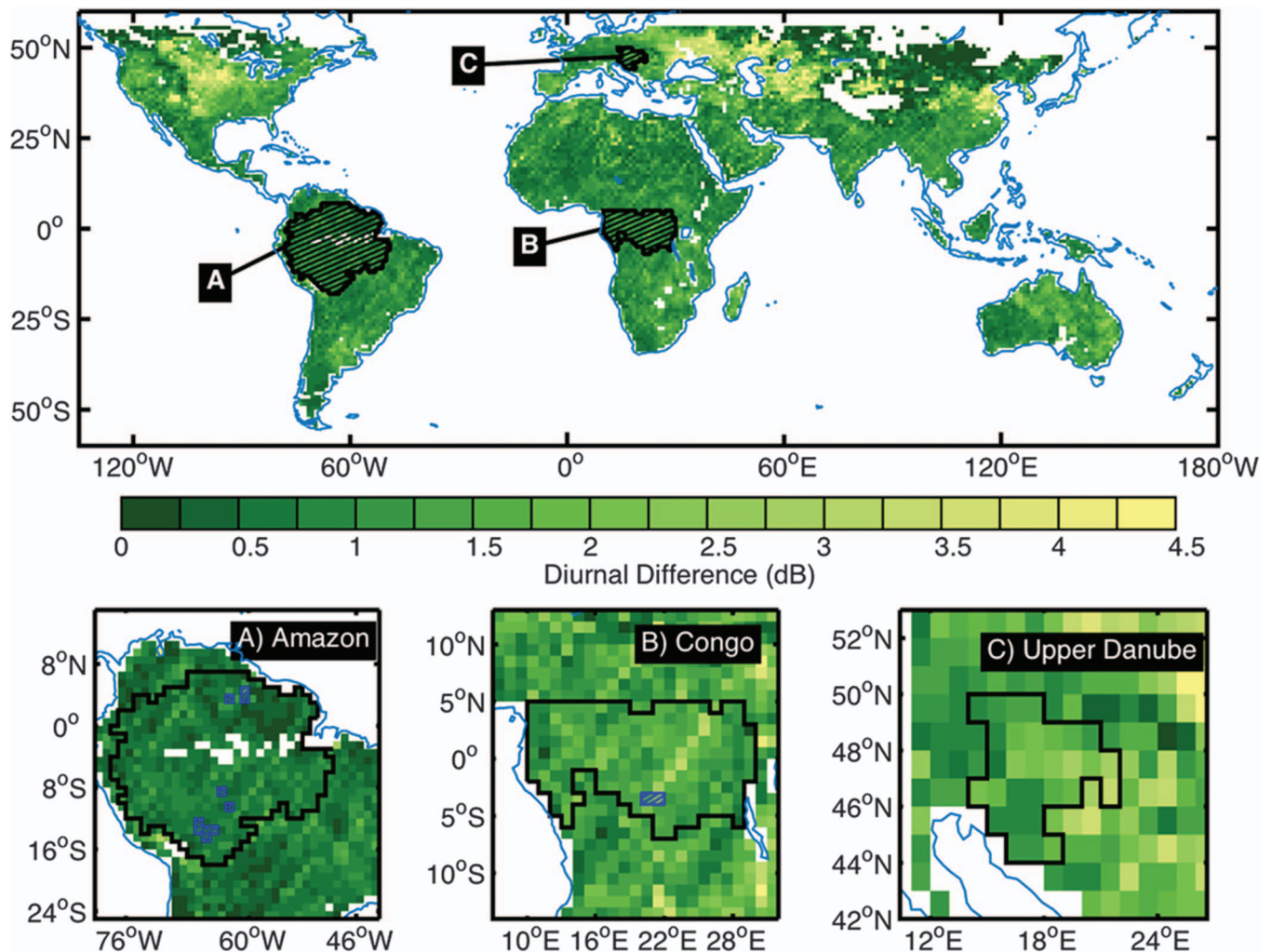
Maps of the diurnal max/min difference of Ku-band RapidScat HH backscatter with three expanded subregions: Amazon, Congo, and Upper Danube.
