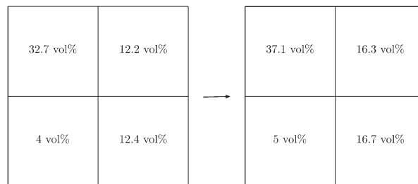
Fig. 8. VIC simulations (left-hand side) and corresponding downscaled SMOS soil moisture (right-hand side) on 17/08/2010 for pixel A (ascending SMOS overpass). All soil moisture contents are expressed as vol%.
