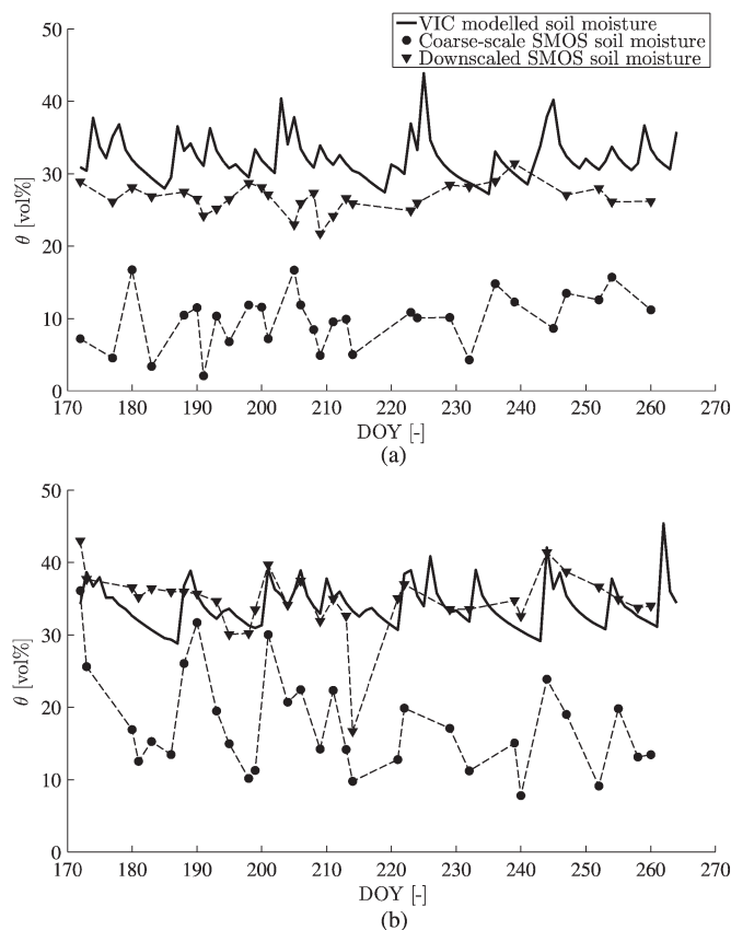
Fig. 13. Time series of soil moisture for one random fine-scale VIC pixel located within the coarse-scale SMOS pixel A (a) and pixel B (b) for the third season (JJA) of the year 2010 (black line), and corresponding SMOS coarse-scale and downscaled soil moisture values.
