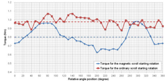
Fig. 7. Experimental results for the torques for starting rotations of the ordinary scroll air motor and the prototype magnetic scroll air motor.
