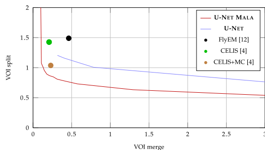
(b) VOI split/merge on FIB-25 (lower is better).
