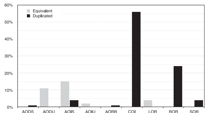
Fig. 4. The proportion of equivalent and duplicated mutants detected by TCE per program studied in case of Java.
