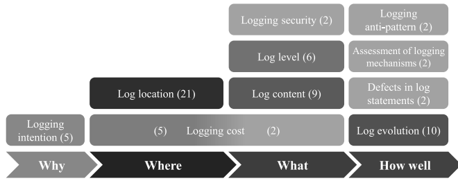
Fig. 7. Relationship between research topics and 3W1H categorization.
