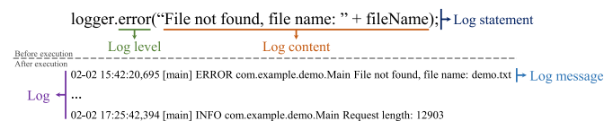
Fig. 1. Logging related terms in an example.
