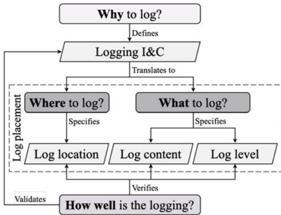
Fig. 5. The relationships between the questions in the 3W1H categorization.
