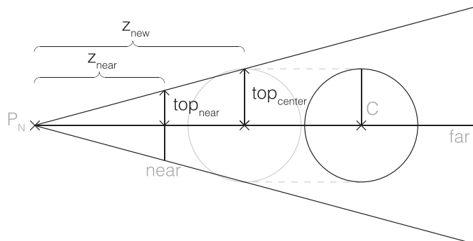
Fig. 7. To show all objects of the current hierarchy level, we enclose them with a bounding sphere. We then move the camera such that the view frustum touches the top (and bottom) points of the bounding sphere.
