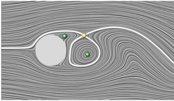
Fig. 4. Flow data depicted with a direct (LIC) visualization that is overlaid with the corresponding topology, i.e., the abstraction of the flow [105]. Image © and courtesy of Tino Weinkauff, used with permission.
