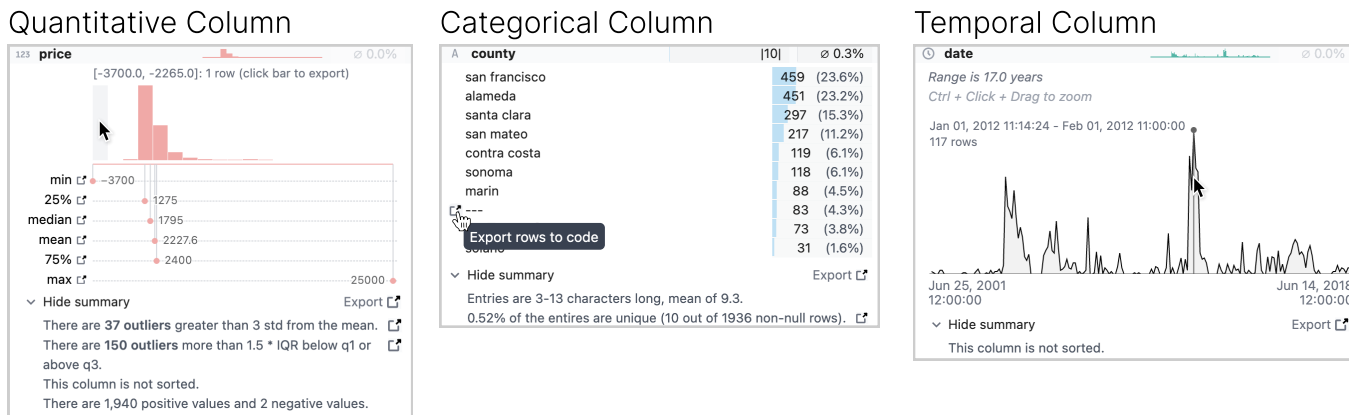
Fig. 2: AutoProfiler shows distributions and summary information depending on the column type. For quantitative columns, we show a binned histogram along with summary statistics. On hover, the user can see the count in each bin or export the selection to code. We also show a summary with extra information like potential outliers that can be exported to code. For categorical columns like strings or boolean values, we show up to the top 10 most frequent values. On click, the selection can also be exported to code. For temporal columns, we show the count of records over time and the range of the column.
