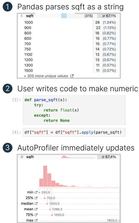
Fig. 3: AutoProfiler updates the data profiles shown as soon as the data updates. In this example, Pandas parses the sqft column as a string type since some of the values initially have strings in them. Once the dataframe df updates in memory, AutoProfiler will update the profile shown. This way the user can see their transformation was successful, inspect the distribution of sqft, and even notice that the number of nulls increased by 0.3% after this parse.
