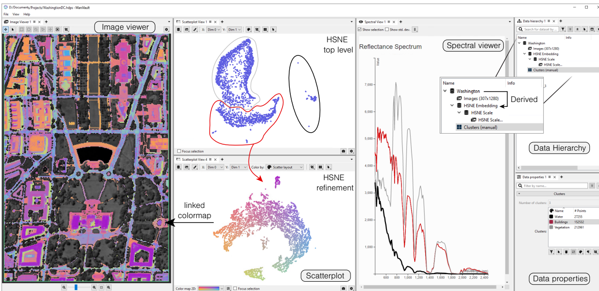
Fig. 1: Example screenshot of ManiVault used for the exploration of a hyperspectral imaging data set.
