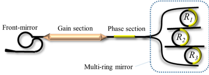
Fig. 1. Schematic structure of a basic widely tunable Si/III-V laser based on multiring mirrors. Here, the three ring resonators are used to illustrate the multiring mirror structure, in which add-drop rings are cascaded within a loop.
