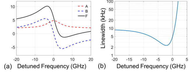
Fig. 7. (a) Calculated values for coefficients A, B and F (a) estimated Lorentzian linewidth as functions of frequency detuned from the dual-ring mirror's resonance frequency assuming an output power of 10 mW. Values of parameters used for these calculations are listed in Table I.
